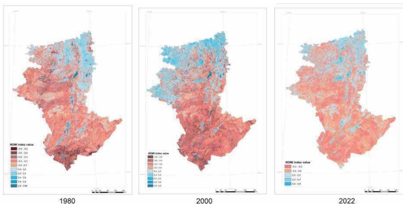
Figure 4. Normalized Difference Moisture Index
