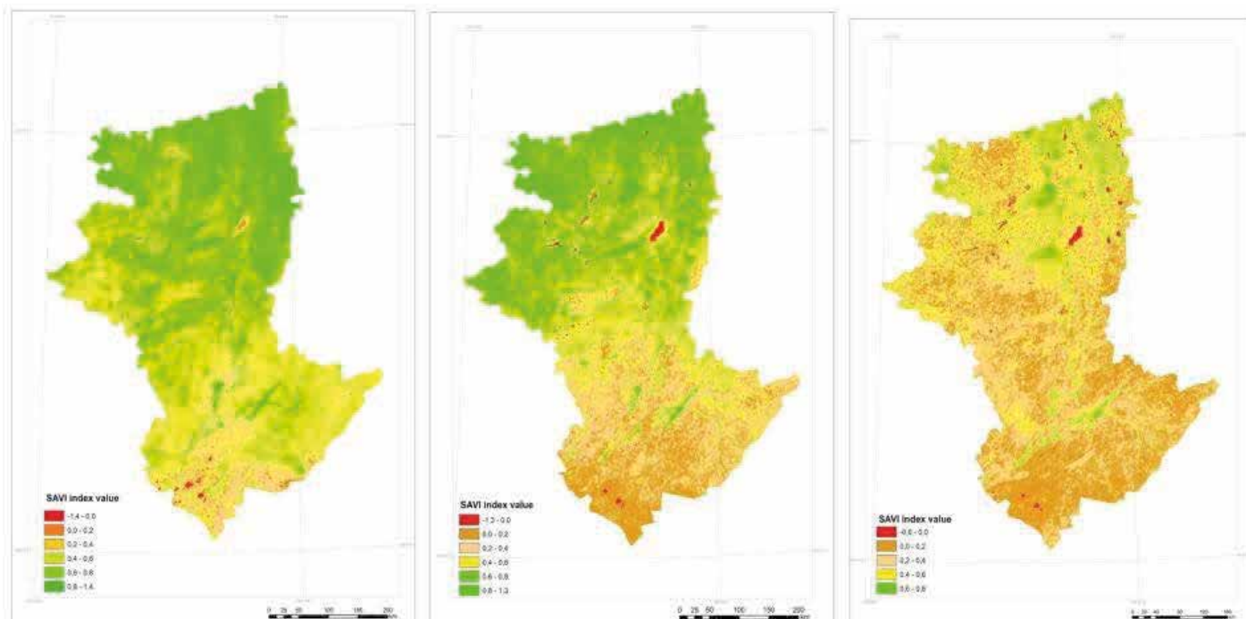
Figure 9. Soil Adjusted Vegetation Index
