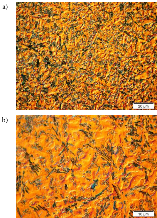
Fig. 1. Microstructure of as-cast experimental AEZ951 magnesium alloy; light microscopy with differential interface contrast
