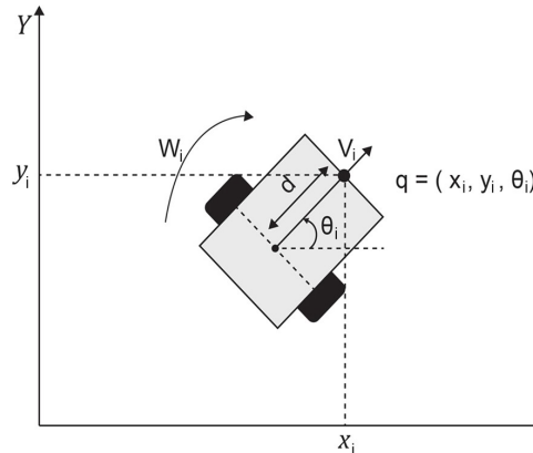
Fig. 1. Nonholonomic mobile robot
