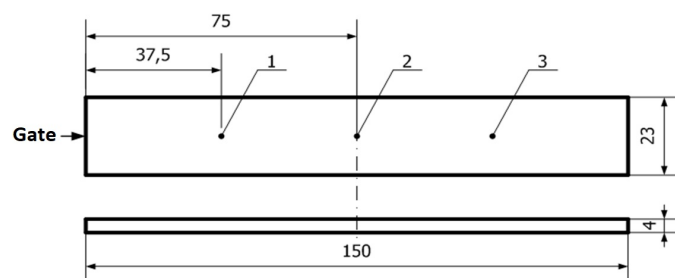
Fig. 4. Molding with marked measuring points
