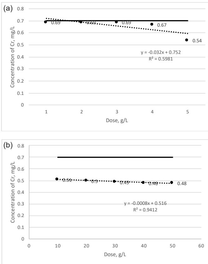
Figure 5. The dependency of Cr concentration on different amounts of sapropele (a) 1, 2, 3, 4, and 5 g/L, (b) 10, 20, 30, 40, and 50 g/L.
