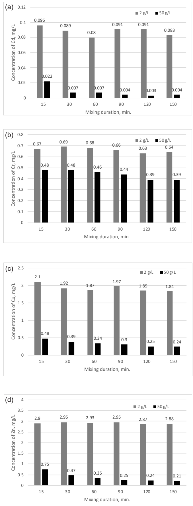
Figure 10. The efficiency of removal of HM from the aqueous solution by using different mixing durations (15, 30, 60, 90, 120, 150 min.) (a) – Cd, (b) – Cr, (c) – Cu, (d) – Zn
