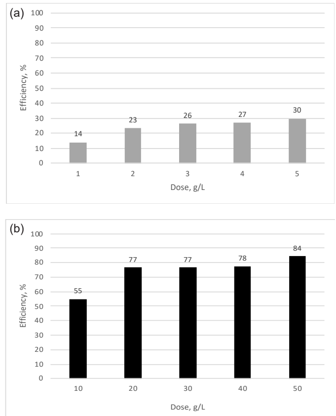
Figure 6. The efficiency of Cu removal from the aqueous solution by using different doses of sapropele (a) 1, 2, 3, 4, and 5 g/L, (b) 10, 20, 30, 40, and 50 g/L.
