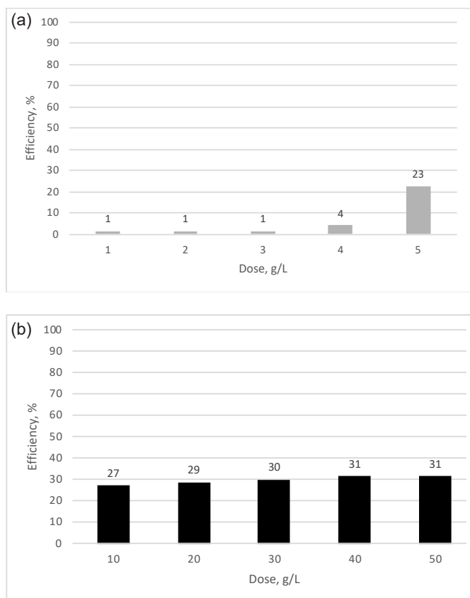
Figure 4. The efficiency of Cr removal from the aqueous solution by using different doses of sapropel (a) 1, 2, 3, 4, and 5 g/L, (b) 10, 20, 30, 40, and 50 g/L.
