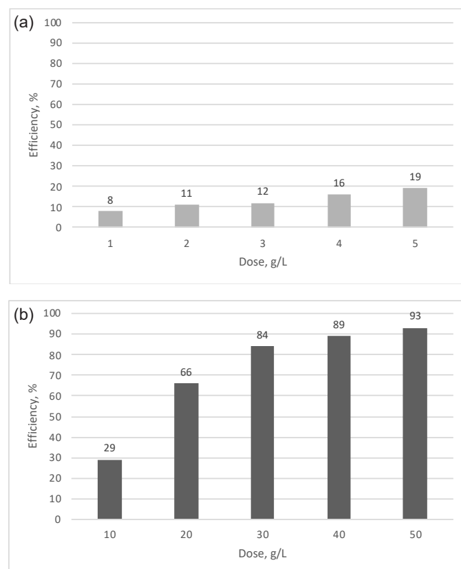
Figure 2. The efficiency of Cd removal from the aqueous solution by using different doses of sapropel (a) 1, 2, 3, 4, and 5 g/L, (b) 10, 20, 30, 40, and 50 g/L.
