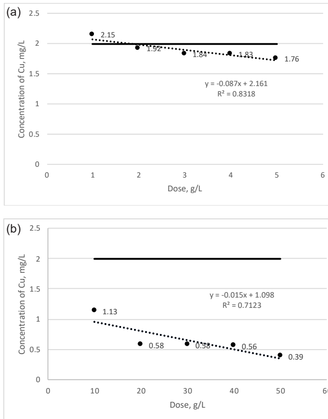
Figure 7. The dependency of Cu concentration on different doses of sapropel (a) 1, 2, 3, 4, and 5 g/L, (b) 10, 20, 30, 40, and 50 g/L.
