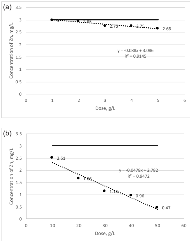
Figure 9. The dependency of Zn concentration on different doses of sapropel (a) 1, 2, 3, 4, and 5 g/L, (b) 10, 20, 30, 40, and 50 g/L.
