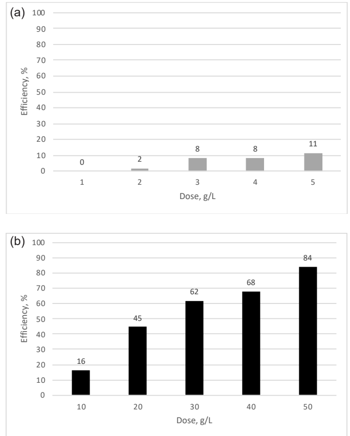
Figure 8. The efficiency of Zn removal from the aqueous solution by using different doses of sapropel (a) 1, 2, 3, 4, and 5 g/L, (b) 10, 20, 30, 40, and 50 g/L.
