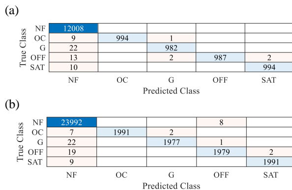
Fig. 9. Confusion matrices for the IM (a) and the PMSM (b)
