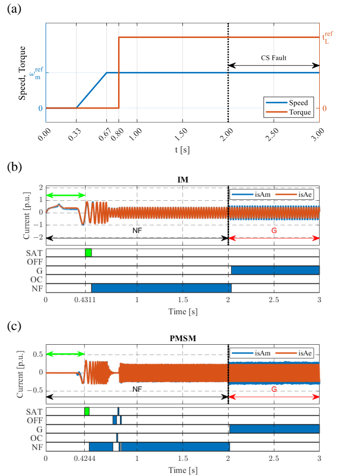
Fig. 7. The waveforms of the set speed and torque and the moment of fault occurrence (a), the waveforms of the currents and the classification results in a drive system with an IM motor (b) and a PMSM motor (c) at a speed of 0.75\omega_{mN} and a load of 0.25t_{LN}
