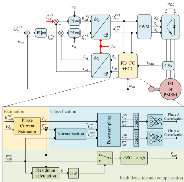
Fig. 1. Schematic diagram of the FOC structure for an IM and PMSM motor including the detection (FD), compensation (FC) and classification (FCL) module
