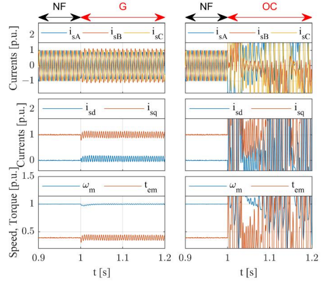
Fig. 5. Waveforms of selected state variables in PMSM when CS faults (G, OC) occur in phase A ( t_L = t_{LN} , \omega_m = \omega_{mN} )
