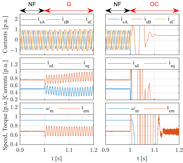
Fig. 3. Waveforms of selected state variables in IM when CS faults (G, OC) occur in phase A ( t_L = t_{LN} , \omega_m = \omega_{mN} )
