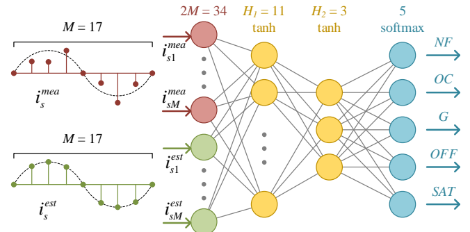
Fig. 6. Schematic diagram of the neural network used
