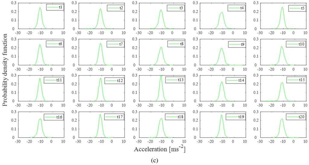
Fig. 5. PDFs of three signals in Control Loop #15. (a) air gap; (b) current; (c) acceleration.
