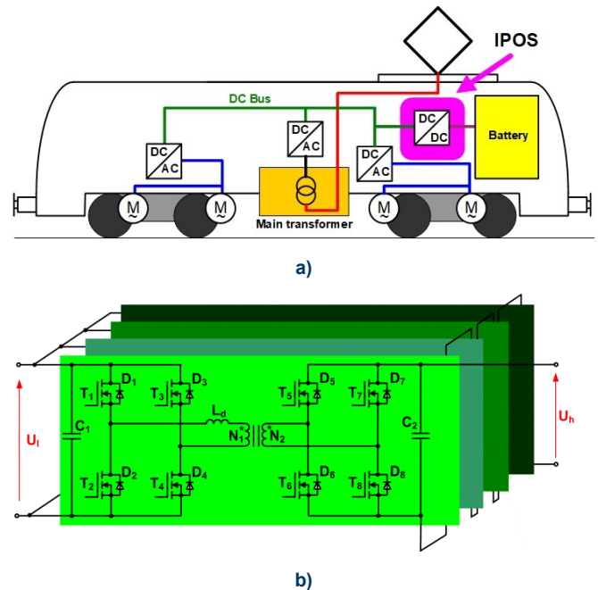
Fig.4. a) concept of an electric locomotive with an additional energy storage tank, b) a modular DC/DC converter in IPOS configuration [15].
