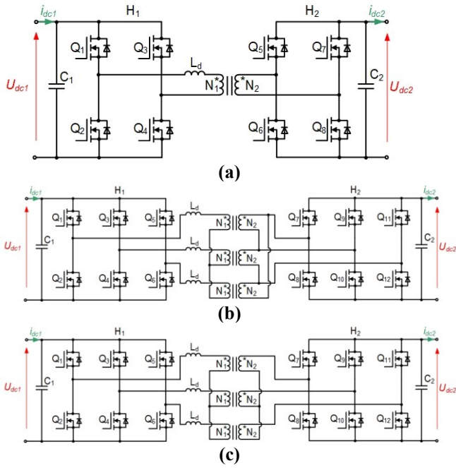
Fig.17. Basic DAB topologies: a) single phase, b) three phase in star-star transformer topology (Y-Y), c) three phase in star-star delta topology (Y-D).
