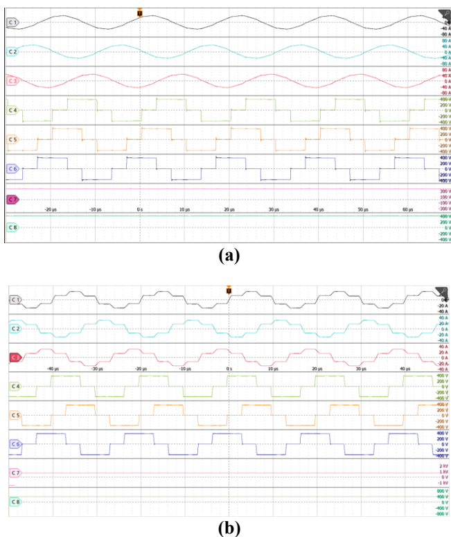
Fig.20. Example operational waveforms of 10 kW three-phase DAB DC/DC converter. From top: C1-C3 phase currents ( I_{1-3} ), C4-6 phase voltages ( U_{1-3} ), C7 – input DC link voltage ( U_{dc1} ), C8 – output DC link voltage ( U_{dc2} ): a) star-delta, b) star-star, 10 \mu s/div.
