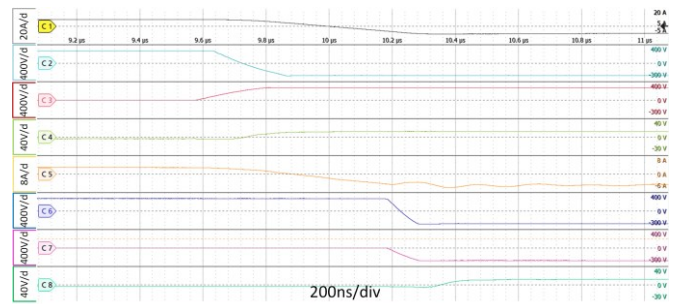
Fig.9. Transistor soft turn-off in a converter bridge leg with additional parallel capacitances. Deeper waveform discussion in [36].
