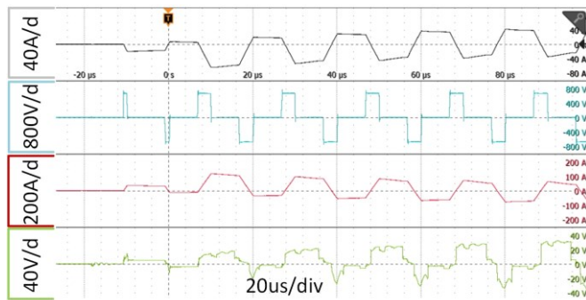
Fig. 15. Starting procedure of DAB. From top: current and voltage in the AC circuit at primary side, current and voltage in the AC circuit at secondary side.
