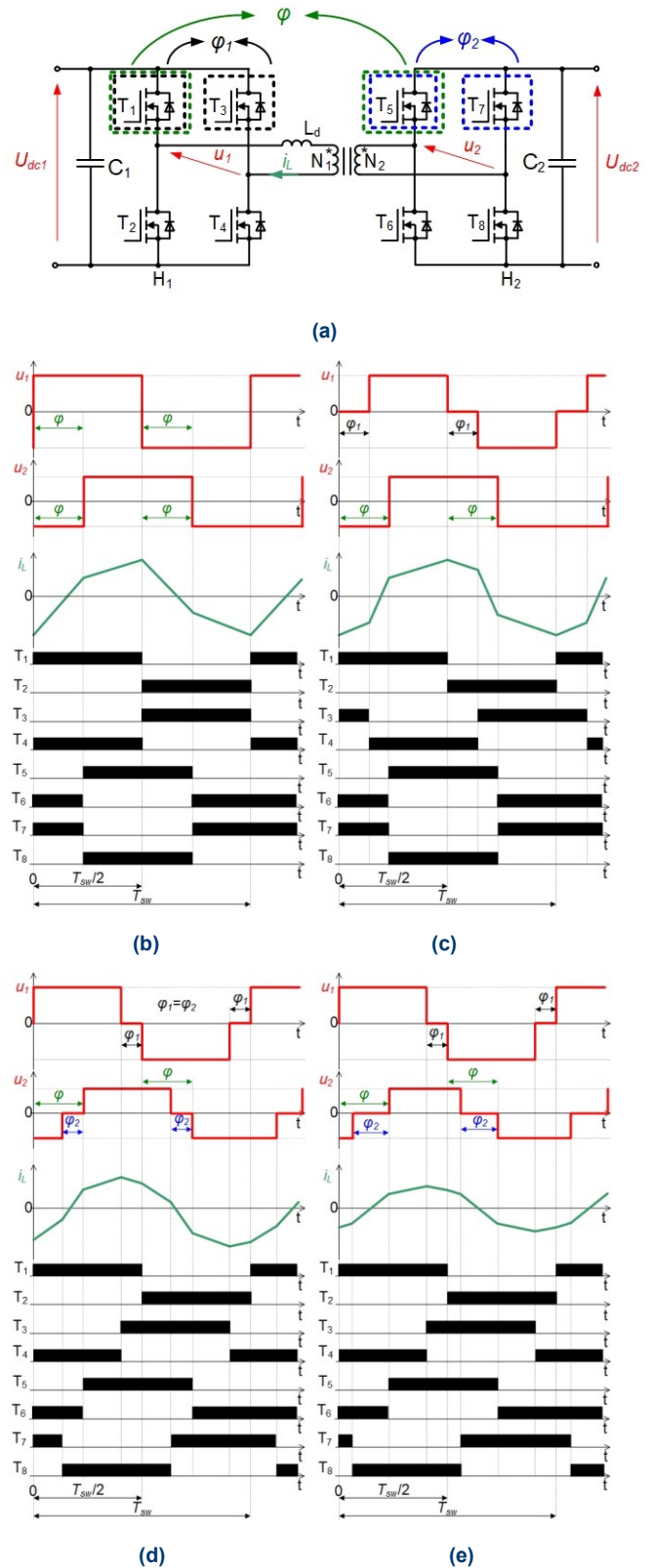
Fig. 8. Control strategies of DAB converter: a) scheme, b) SPS, c) EPS, d) DPS, e) TPS.
