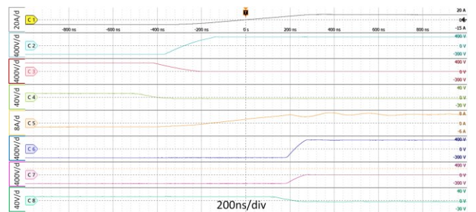
Fig.11. Soft switching of DAB transistors (transistors' designations as in the fig. 2), a) rising edge of the upper transistor, b) falling edge of the upper transistor. From the top: C1 – current of the primary side series inductor L_d ( I_1 ), C2 – voltage of the primary side transformer ( U_1 ), C3 –voltage of the transistor T1 drain-source ( U_{c1} ), C4 – gate voltage of the transistor T2 drain-source ( U_{c2} ), C5 –current of the secondary side transformer ( I_2 ), C6 –voltage of the secondary side transformer ( U_2 ), C7 – voltage of the transistor T5 drain-source, C8 – gate voltage of the transistor T6 drain-source, 200ns/div and 4us/div.
