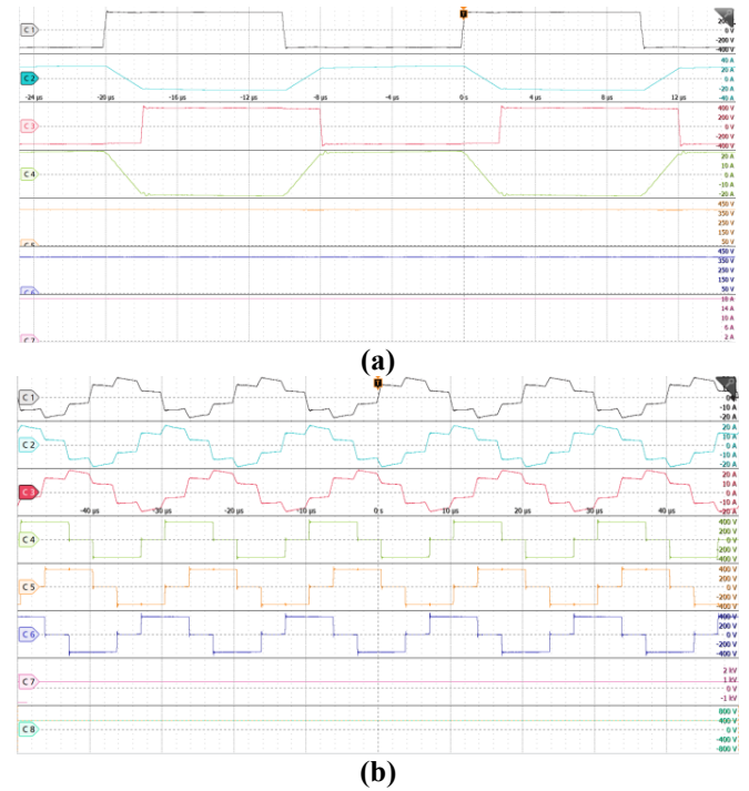
Fig.18. Experimental waveforms of DAB DC/DC converter: a) single-phase configuration. From top: C1-2 primary phase voltage and current ($U_1, I_1$), C2-3 secondary phase voltage and current ($U_2, I_2$), C7 - input DC link voltage ($U_{dc1}$), C8 - output DC link voltage ($U_{dc2}$); b) three-phase star-star configuration. From top: C1-C3 phase currents ($I_{1-3}$), C4-6 phase voltages ($U_{1-3}$), C7 - input DC link voltage ($U_{dc1}$), C8 - output DC link voltage ($U_{dc2}$), 10us/div.
