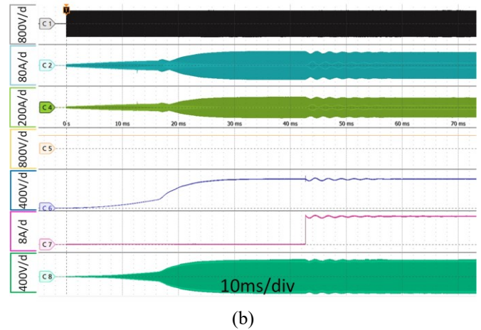
Fig. 16. DAB converter inrush current limitation method proposed in [42]. a) without inrush current limitation, from top: C1 – primary phase voltage ( U_1 ), C2 – primary phase current ( I_1 ), C3 – secondary phase voltage ( U_2 ), C4 – secondary phase current ( I_2 ), C5 – DC input voltage ( U_{dc1} ), C6 – DC output voltage ( U_{dc2} ), b) with inrush current limitation, from top: C1 – primary phase voltage ( U_1 ), C2 – primary phase current ( I_1 ), C3 – secondary phase voltage ( U_2 ), C4 – secondary phase current ( I_2 ), C5 – DC input voltage ( U_{dc1} ), C6 – DC output voltage ( U_{dc2} ), C7 – DC output current ( I_{dc2} ), C8 – secondary phase voltage ( U_2 ).
