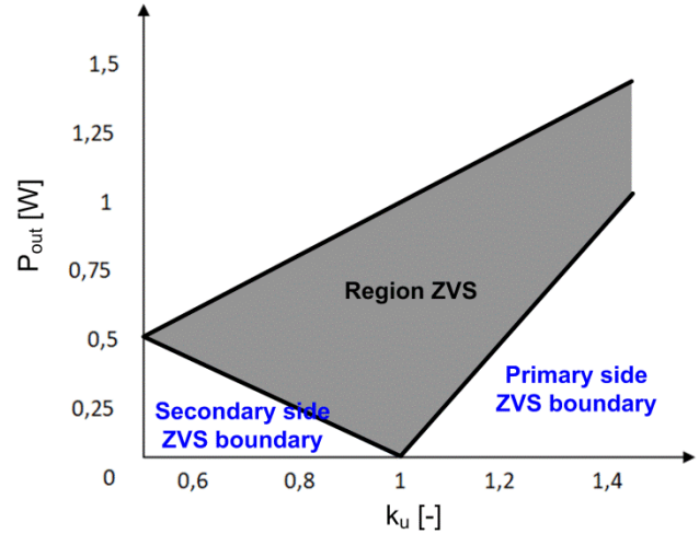
Fig.10. Zero Voltage Switching (ZVS) region characteristic.
