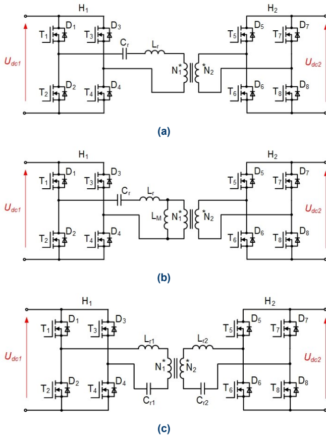
Fig.6. Different resonant DAB converters: a) DAB-SRC [23], b) DAB-LLC [24], c) DAB-CLLC configuration with symmetrical resonant tank [26].
