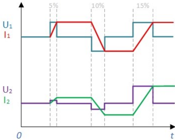
Fig. 14. DAB converter inrush current limitation method proposed in [42].
