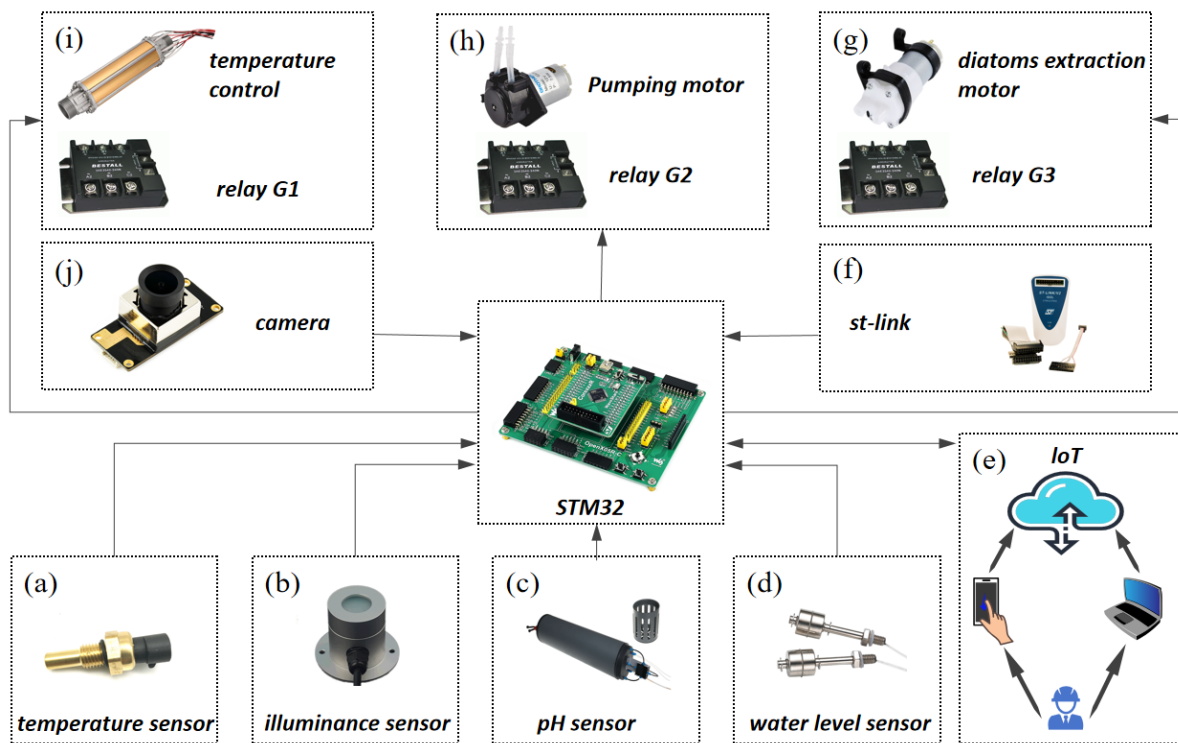
Fig. 8. Regeneration system for sodium silicate used sands
