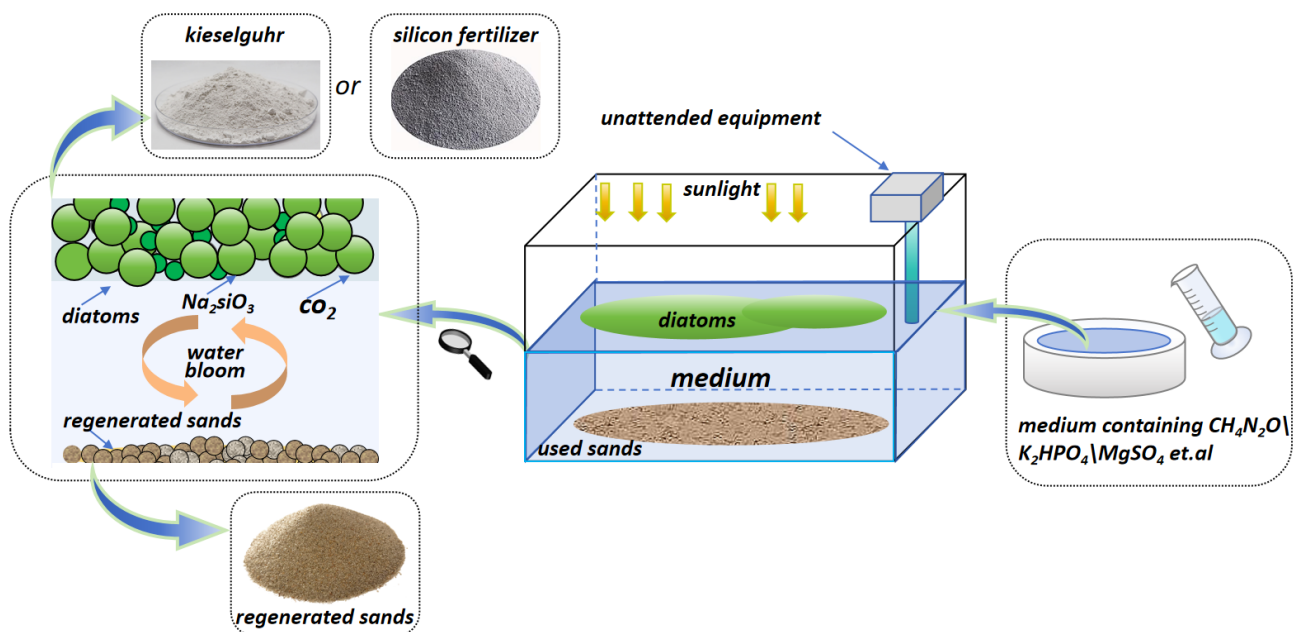
Fig. 1. Bio-regeneration method for sodium silicate used sands
