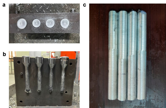
Fig. 1. Images of (a) solidification in a metal die (b) cast rods (c) machined rods
