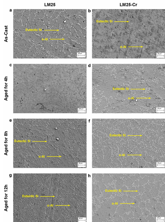
Fig. 3. Microstructure of the specimens (Scanning Electron Microscopy)
