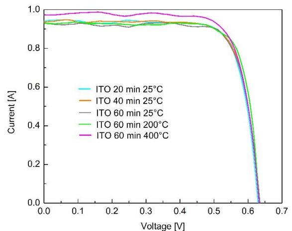
Fig.11. Current-voltage characteristics of the polycrystalline silicon photovoltaic cells with ITO layer deposited by the PVD method.
