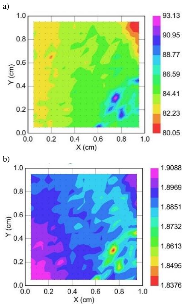
Fig.10. Thickness (a) and refractive index (b) distribution maps for ITO layers deposited at 400°C in 60 min.
