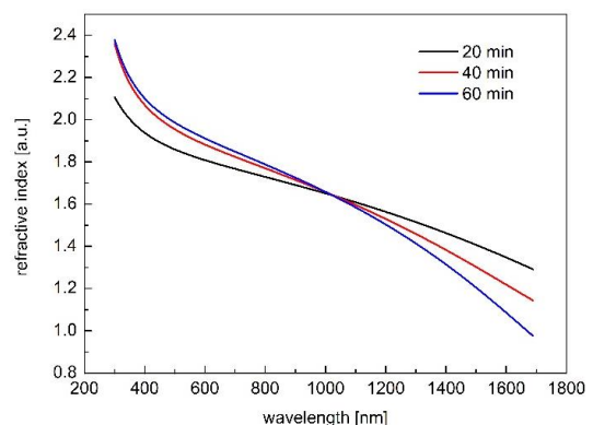
Fig.8. Dispersion dependences of the refractive index of ITO layers deposited with 400°C on a substrate in the form of glass plate
