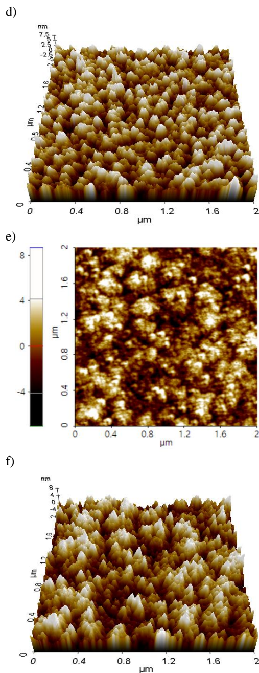
Fig.5. The AFM image of the surface morphology of the ITO thin film and its 3D representation deposited after 60 minutes with different temperature in °C: 25 (a+b); 200 (c+d); 400 (e+f)
