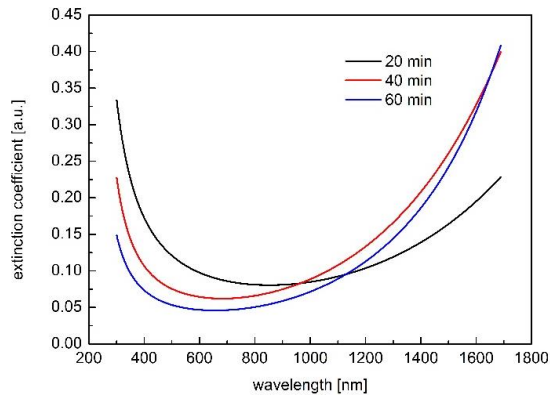
Fig.9. Dispersion dependences of the extinction coefficient of ITO layers deposited with 400°C on a substrate in the form of glass plate
