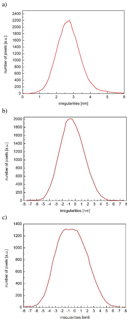
Fig.6. The histogram of frequencies with the occurred heights for ITO thin films deposited with different temperature in °C: a) 25; b) 200; c) 400
