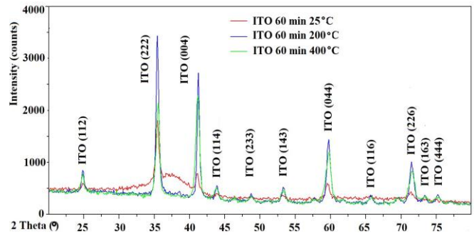
Fig.7. The diffraction patterns of ITO thin films deposited with different temperature
