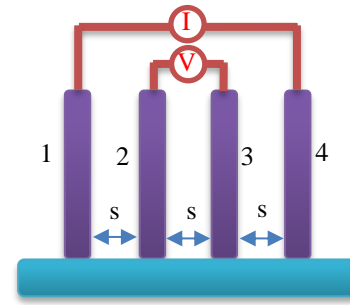
Fig.2. The principle of operation of four-point probe in a schematic view
