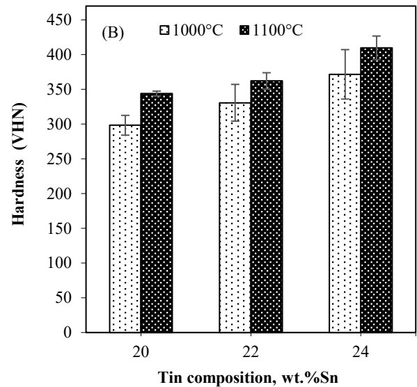
Fig.9. Mechanical properties (A) tensile strength of Cu-Sn (B) hardness of Cu-Sn
