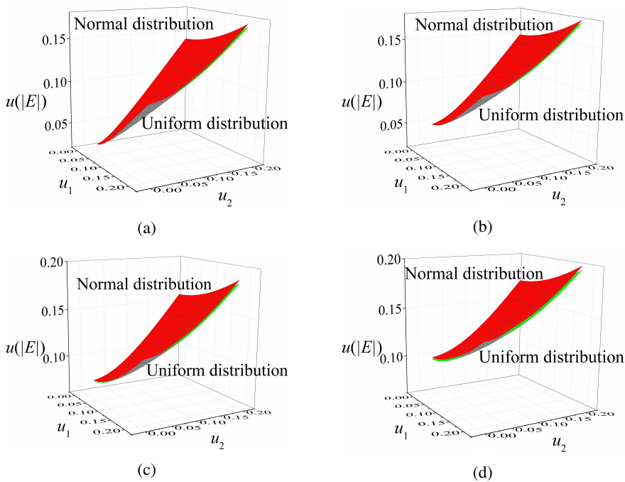
Fig. 2. Comparison of the uncertainties of magnitude with the uniform distribution and normal distribution ( \theta = \varphi = \pi/4 ): (a) u_3 = 0.05 ; (b) u_3 = 0.1 ; (c) u_3 = 0.15 ; (d) u_3 = 0.2 .
