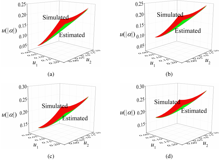
Fig. 6. Comparison of the uncertainties of the polarization direction obtained by the GUM method and the MCM method ( \theta = \varphi = \pi/4 ): (a) u_3 = 0.05 ; (b) u_3 = 0.1 ; (c) u_3 = 0.15 ; (d) u_3 = 0.2 .
