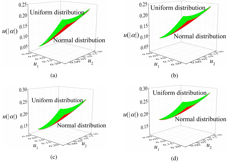
Fig. 3. Comparison of uncertainties of the polarization direction with the uniform distribution and normal distribution ( \theta = \varphi = \pi/4 ): (a) u_3 = 0.05 ; (b) u_3 = 0.1 ; (c) u_3 = 0.15 ; (d) u_3 = 0.2 .
