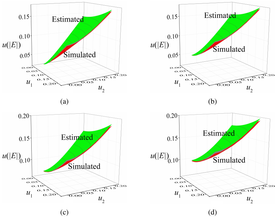
Fig. 5. Comparison of the uncertainties of the magnitude obtained by the GUM method and the MCM method ( \theta = \varphi = \pi/4 ): (a) u_3 = 0.05 ; (b) u_3 = 0.1 ; (c) u_3 = 0.15 ; (d) u_3 = 0.2 .
