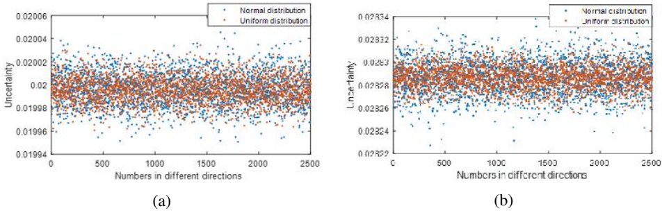
Fig. 4. Uncertainties obtained by MCM method ( u_1 = u_2 = u_3 = 0.2 ): (a) uncertainty of the magnitude; (b) uncertainty of the polarization direction.
