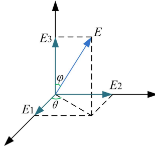
Fig. 1. The spherical coordinate and the rectangular coordinate.
