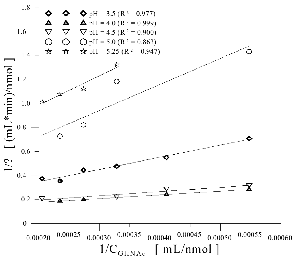
Figure 1. The Lineweaver-Burke plot for enzymatic deacetylation of chitosan; C_{enz} = 0.057 nmol/mL.
