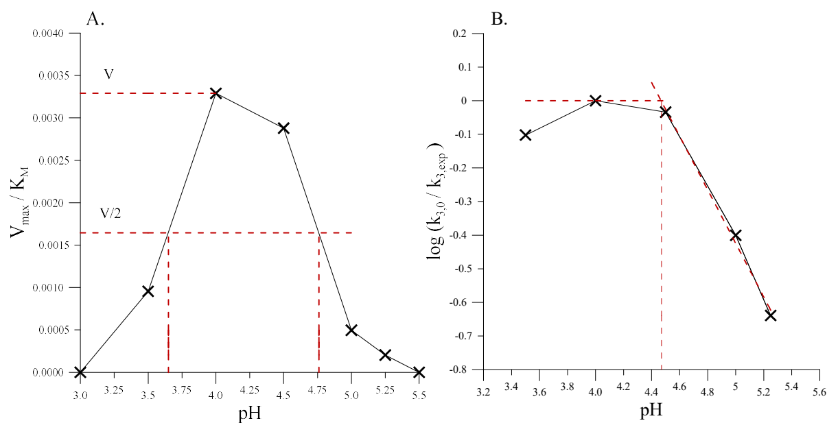
Figure 2. Evaluation of pKa values of amino acids present in the activity center according to Dixon and Webb method (A) and Taylor method (B).
