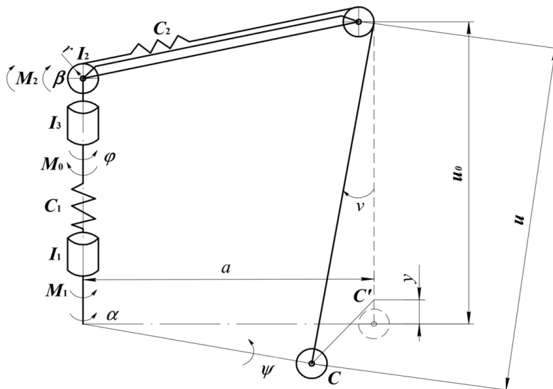
Fig. 1. Dynamic model of the boom system with joint movement of the slewing and hoisting mechanisms
