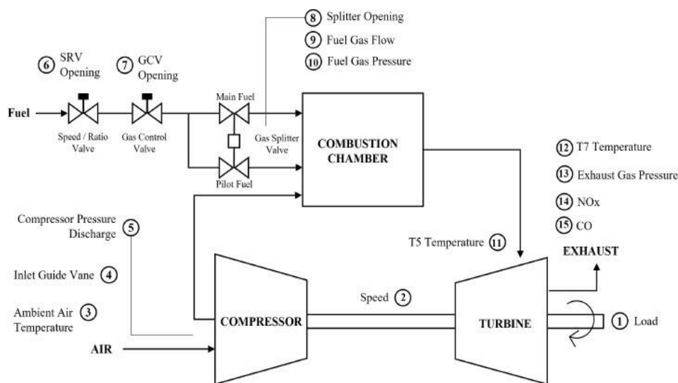
Fig. 3. Flow diagram of the DLE gas turbine
