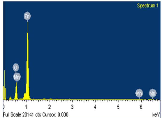
Figure 3. EDX spectrum of Mn-doped ZnO nanoparticles.
