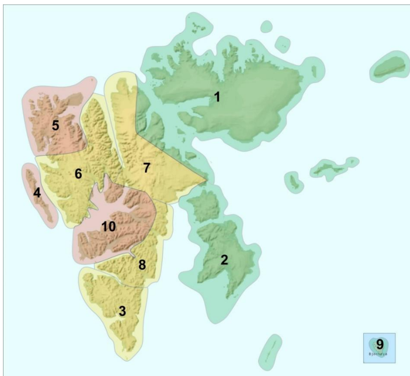
Fig. 1. Cumulative index of environmental change in marine and coastal Svalbard management areas, based on environmental change maps by Węslawski and Urbański (2024). Areas in red (4, 5, 10) are the most impacted, in yellow (3, 6, 7, 8) are moderately changed and in green (1 and 2) are the least impacted; see Table 5.
