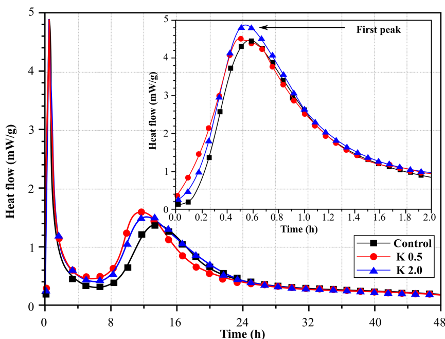
Fig. 4. Heat evolution of alkali activation of slag with incorporation of K-A-S-H nanoparticles [27]
