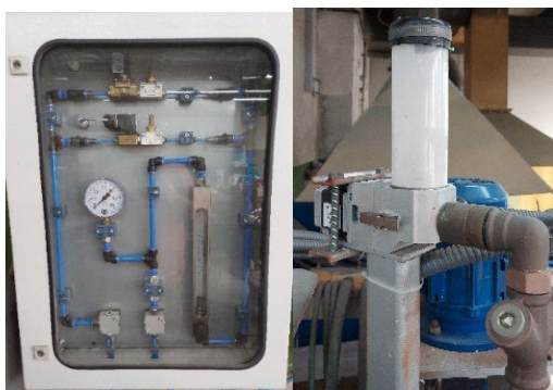
Fig. 2. Refining gas-dispensing system and powder flux dispenser in rotary degassing system
