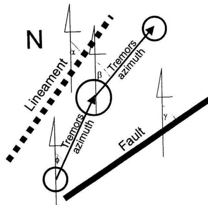
Fig. 3. Parameters applied to statistical analysis of lineament dependence on high energy seismicity \alpha – azimuth of the nearest lineament; \beta – tremor vector azimuth (TVAA), the vector initial point was the epicenter of strong tremors with energy greater than E \geq 10^8 J, and the terminal point was the epicenter strong tremors with energy greater than E \geq 5.5 \cdot 10^5 J but less than 10^8 J; \gamma – azimuth of the nearest fault; \phi – tremor vector azimuth (TVAB), the vector initial point was the epicenter of strong tremors with energy greater than E \geq 5.5 \cdot 10^5 J but less than 10^8 J, and the terminal point was the epicenter of strong tremors with energy greater than E \geq 10^8 J
