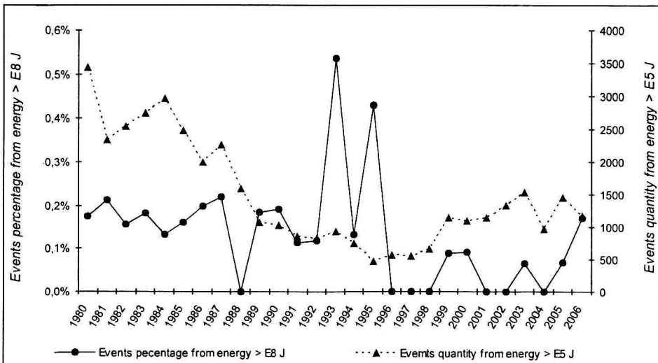
Fig. 1. Amount of high energy tremor distribution in the USB from 1980 to 2006
