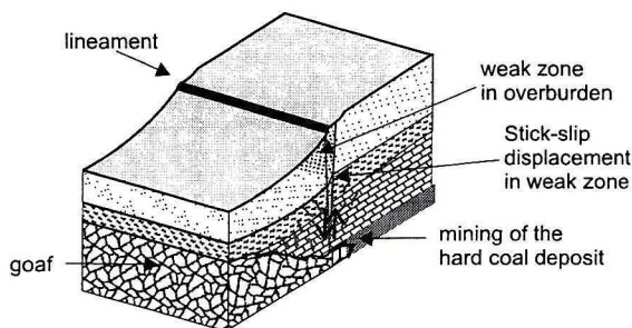
Fig. 2. Lineament which appears as a result of mining (Pilecka et al. 2006)
