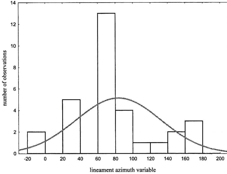
Fig. 6. Histogram of the lineament azimuth variable (for the Upper Silesian Basin – USB)
