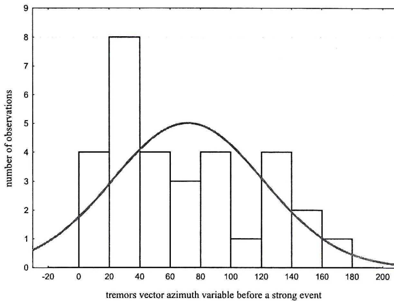
Fig. 4. Histogram of the tremor vector azimuth variable tremor (TVAB) (for the Upper Silesian Basin – USB)
