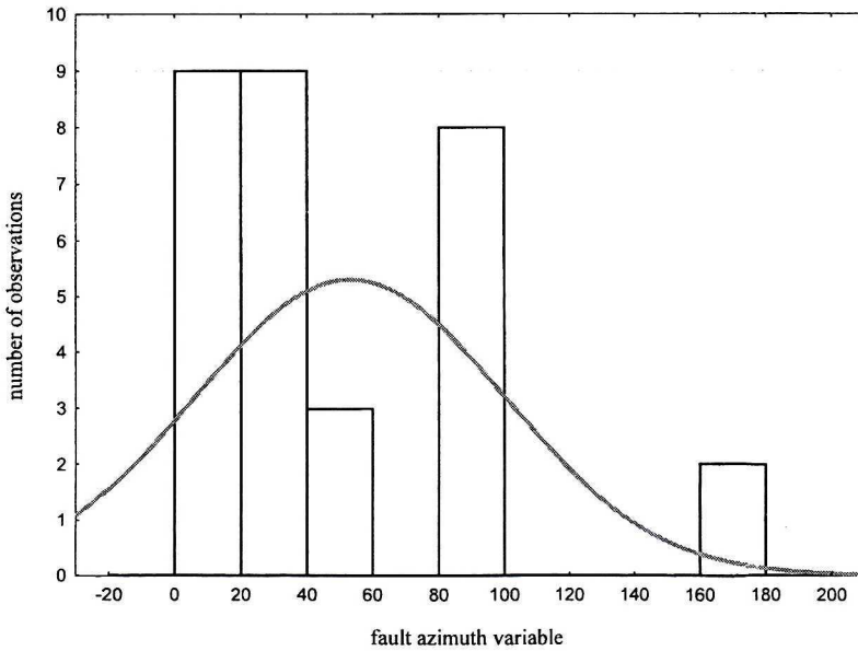
Fig. 7. Histogram of the fault azimuth variable (for the Upper Silesian Basin – USB)
