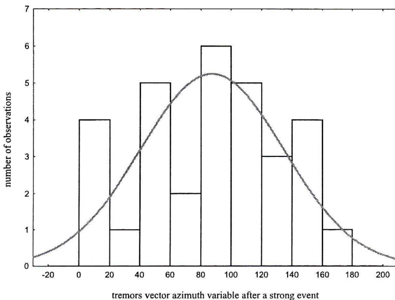
Fig. 5. Histogram of the tremor vector azimuth variable tremor (TVAA) (for the Upper Silesian Basin – USB)
