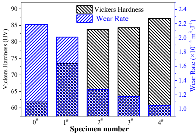
Fig. 16. Wear rate and microhardness of samples
