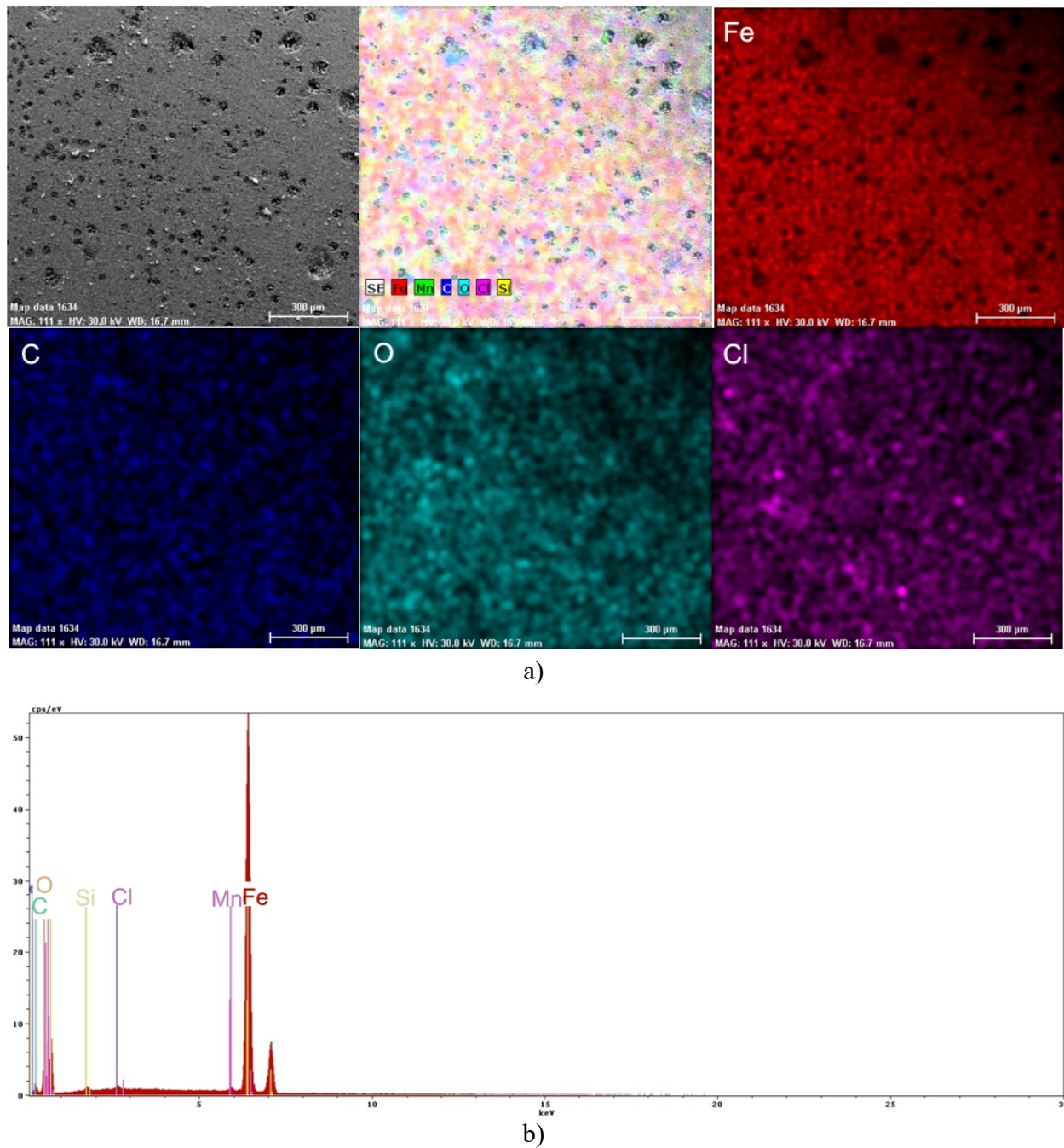
Fig. 11. a) SEM and EDX analysis of CMC corroded steel sample, b) EDX spectrum
