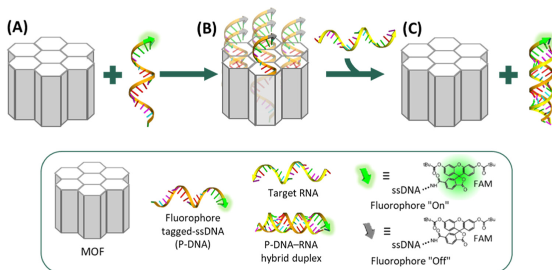
Figure 11. Scheme of the fluorescence quenching-regeneration mechanism of viral RNA detection using a MOF-based sensing platform. Reprinted with permission from (Hadyński et al., 2023). Copyright © 2023 American Chemical Society.
