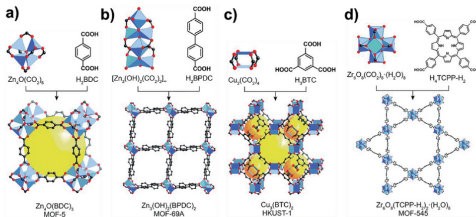
Figure 1. Exemplary MOF structures. Reproduced with permission of Royal Society of Chemistry from (Rungtaweeworant et al., 2017); permission conveyed through Copyright © Clearance Center, Inc.
