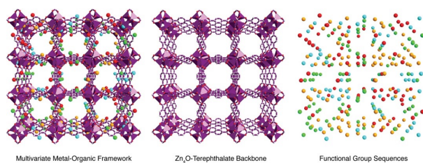
Figure 10. MTV-MOF-5 decomposed into a compositionally and structurally periodic backbone (purple) and an aperiodic decoration of the backbone by four different hypothetical functional groups (red, blue, green, and yellow spheres). Reprinted with permission from (Osborn Popp and Yaghi, 2017). Copyright © 2017 American Chemical Society.
