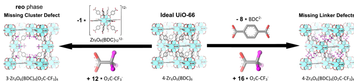
Figure 9. Diagram illustrating the structure and composition differences between ideal and defective UiO-66 unit cells. Reprinted with permission from (Shearer et al., 2016). Copyright © 2016 American Chemical Society.
