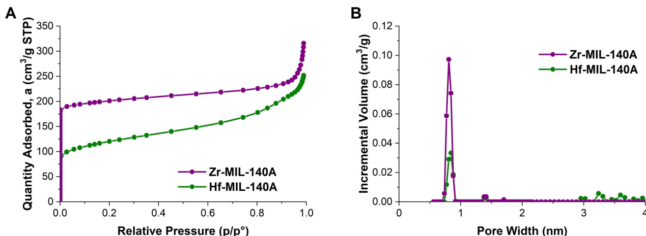
Figure 7. N 2 adsorption isotherms (A) and DFT pore size distribution of MIL-140A samples (B) (Jodłowski et al., 2023b).
