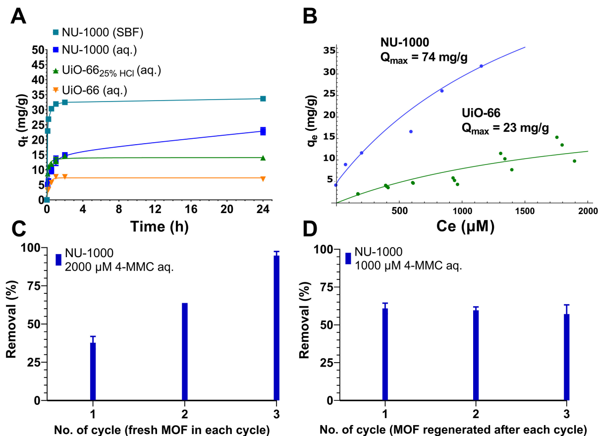
Figure 18. 4-MMC removal efficiency on prepared Zr-MOFs (A), equilibrium loading in prepared Zr-MOFs (B), 4-MMC cascade removal efficiency on NU-1000 (C) (Jodłowski et al., 2023a). Copyright © 2023 Jodłowski P.J., Dymek K., Kurowski G., Hyjek K., Boguszewska-Czubara A., Budzyńska B., Pajdak A., Kuterasiński Ł., Piskorz W., Jeleń P., Sitarz M. Licensed under CC BY 4.0.
