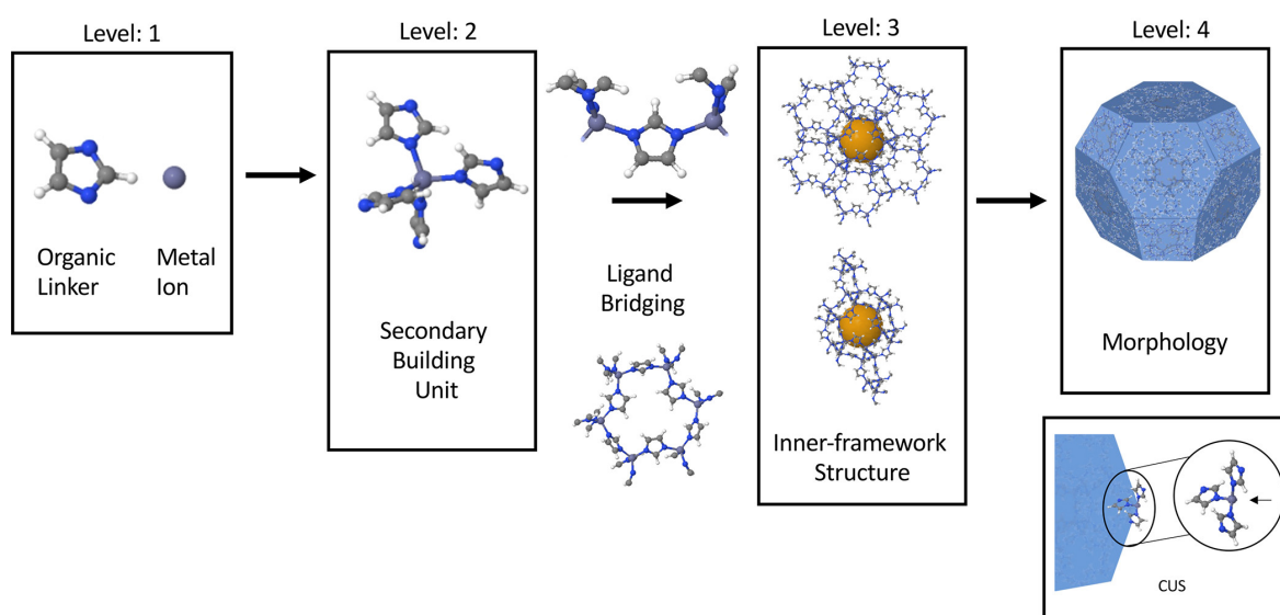
Figure 2. The levels of metal-organic frameworks structure. Reprinted with permission from (Lawson et al., 2021). Copyright © 2021 American Chemical Society.
