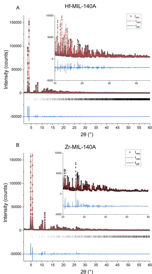
Figure 6. Rietveld plots for MIL-140A with Hf and Zr as a metallic node (Jodłowski et al., 2023b). Copyright © 2023 Jodłowski P.J., Kurowski G., Dymek K., Oszałka M., Piskorz W., Hyjek K., Wach A., Pajdak A., Mazur M., Rainer D.N., Wierzbicki D., Jeleń P., Sitarz M. Licensed under CC BY 4.0.
