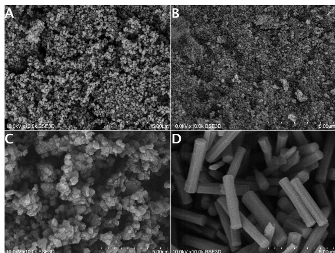
Figure 8. SEM microphotographs of acriflavine@MOF composites: ACF@MOF-808 (A), ACF@UiO-66 (B), ACF@UiO-67 (C), ACF@NU-1000 (D) (Jodłowski et al., 2022).
