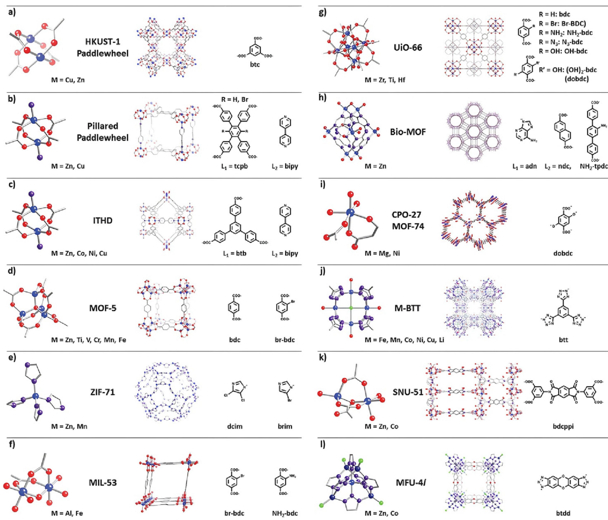
Figure 4. Framework structures (center) and the corresponding secondary building units (SBUs) of some of the most commonly used MOFs (Deria et al., 2014). Copyright © 2014 Deria P., Mondloch J.E., Karagiari O., Bury W., Hupp J.T., Farha O.K. Licensed under CC BY 4.0.
