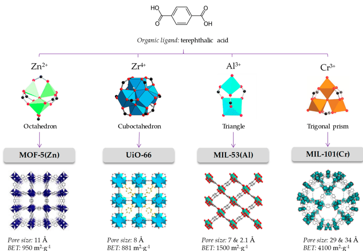
Figure 3. Diverse metal-organic framework based on a common ligand (Rocío-Bautista et al., 2019). Copyright © 2019 Rocío-Bautista P., Taima-Mancera I., Pasán J., Pino V. Licensed under CC BY 4.0.
