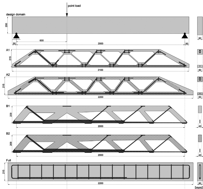
Fig. 9. Concrete girders designed with TO-based STM by two research groups, source: [11]
