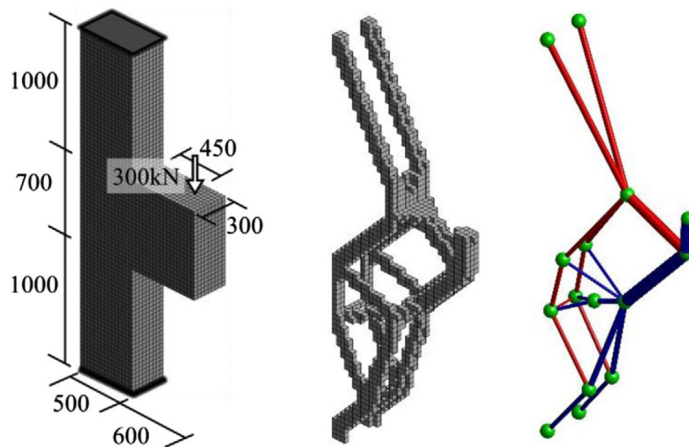
Fig. 8. 3D ST model for corbel generated with TO methods, source [36]
