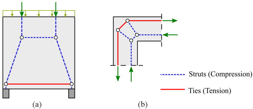
Fig. 2. Examples of ST models; (a) for a deep beam (based on [9]), (b) for a frame corner subjected to the opening moment (based on [12])
