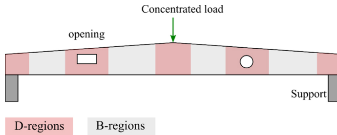
Fig. 1. Illustrative division of a roof girder with openings into B- and D-regions
