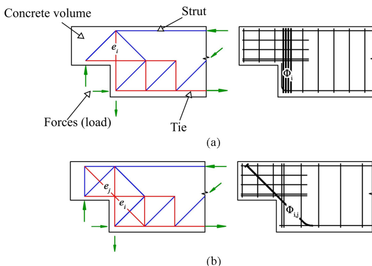
Fig. 6. ST models and corresponding reinforcement layouts obtained with Mozaffari's code for the support zone of a simply supported beam with an undercut; (a) reference solution, (b) modified solution with an additional diagonal bar, source [26]
