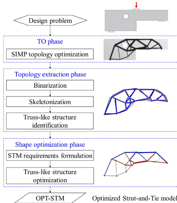
Fig. 7. Flowchart of generating truss-like structure based on TO, source: [35]
