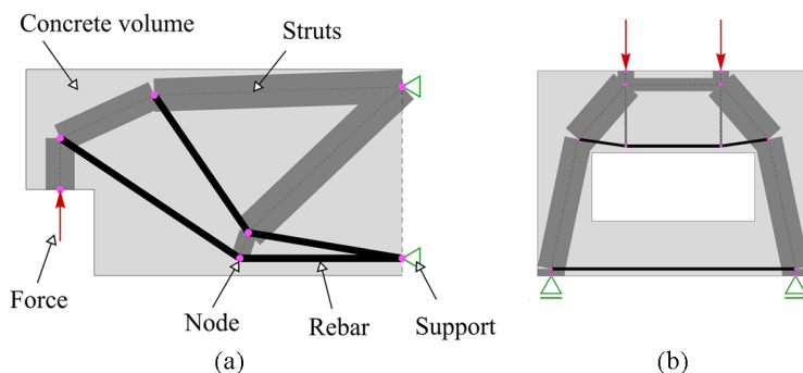
Fig. 5. ST layouts obtained with Bołbotowski's code; (a) support zone of a simply supported beam with an undercut, (b) a plate with an opening, source [25]
