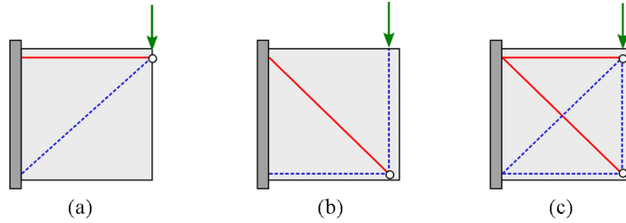
Fig. 4. Introductory example of different ST models from [18], description in the text
