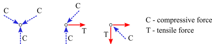
Fig. 3. Basic types of nodes according to Eurocode 2 [12]
