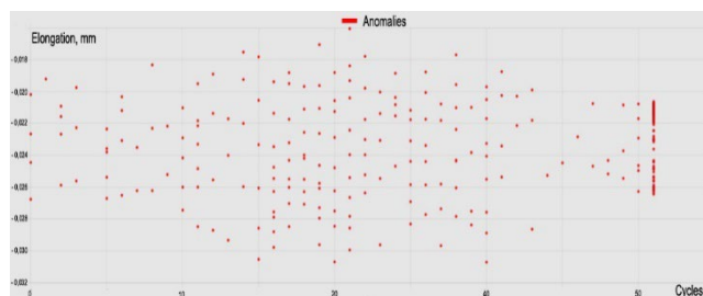
Fig. 4. Elongation anomaly graph from cycles for the worm8 sample determined using the Isolation Forest algorithm
