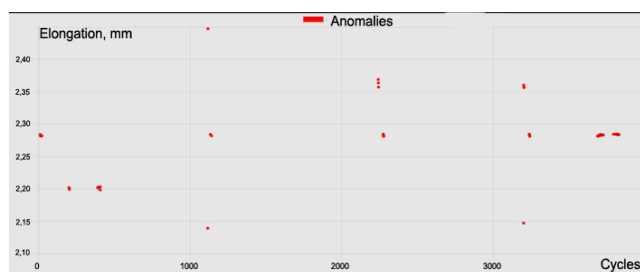
Fig. 5. Elongation anomaly graph from cycles for sample WP1 determined using the One-Class SVM algorithm
