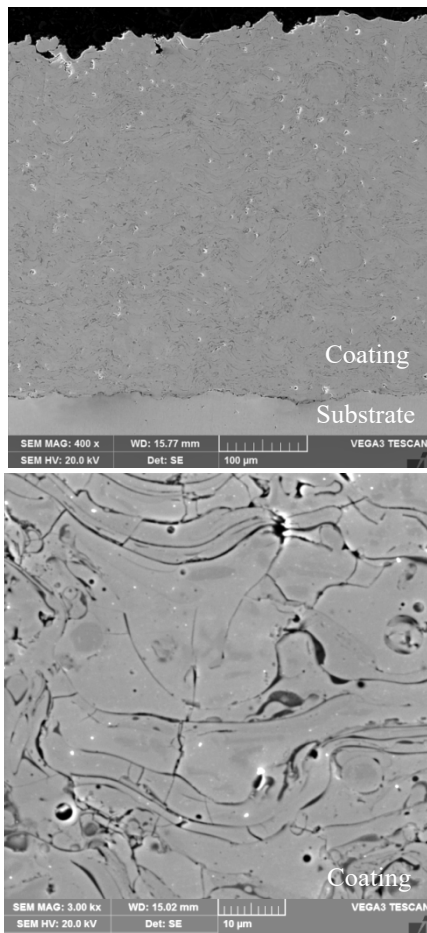
Fig. 6. Example view of the CrNi coating thermally sprayed using the APS method on a P250GH steel substrate, with an average thickness of 403 µm
