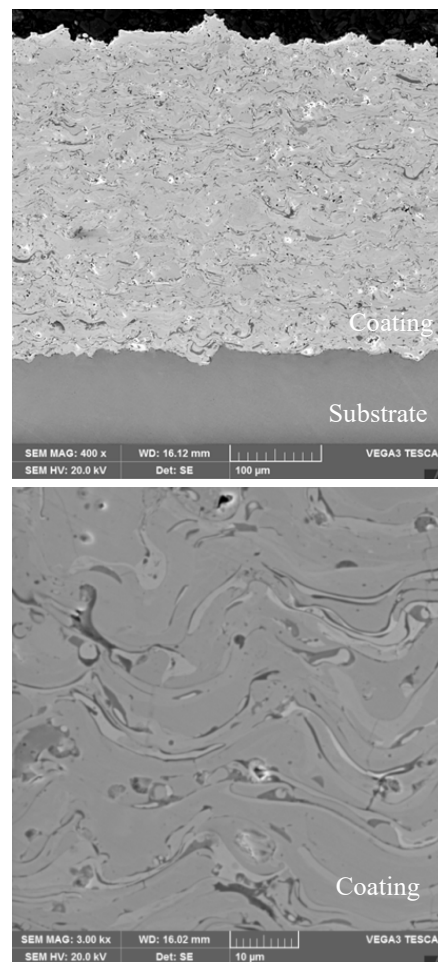
Fig. 5. Example view of the WCCoCr coating thermally sprayed using the APS method on a P250GH steel substrate, with an average thickness of 348 \mu\text{m}
