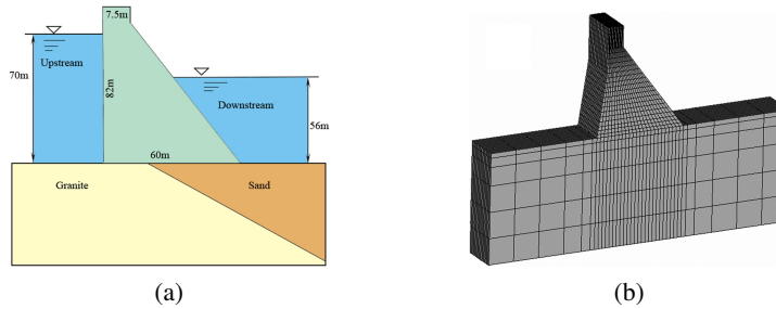
Fig. 2. Concrete dam and model: (a) The profile map of the dam body in this study, (b) Finite element calculation model of this study
