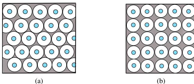
Fig. 5. Cold water pipe layout scheme: (a) The plum flower form layout scheme, (b) Rectangle scheme
