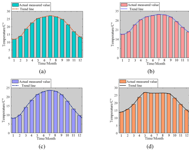
Fig. 3. Temperature parameters: (a) Average temperature, (b) Average maximum temperature, (c) Average minimum temperature, (d) Average river temperature
