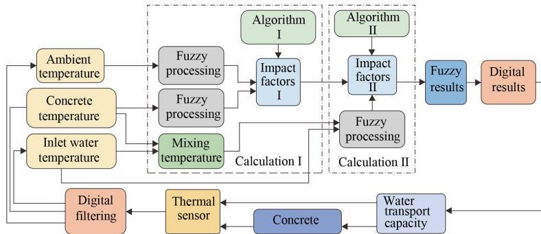
Fig. 12. Temperature control algorithm flowchart
