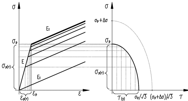
Fig. 10. Set of characteristics on idealised stress-strain diagram – influence of shear stress on normal stress at which yielding limit in space (\sigma, \tau) is obtained (own elaboration)
