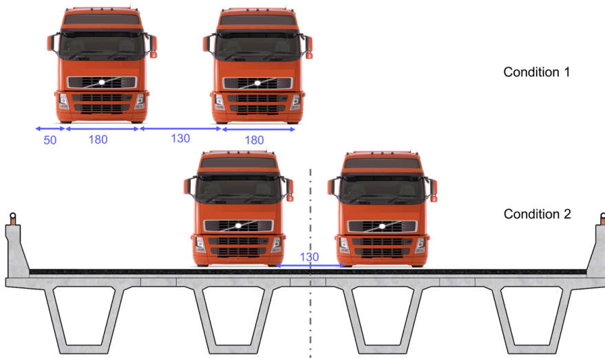
Fig. 7. Schematic diagram of vehicle arrangement for load test condition
