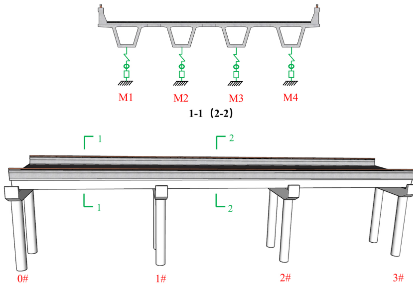
Fig. 6. Test section diagram
