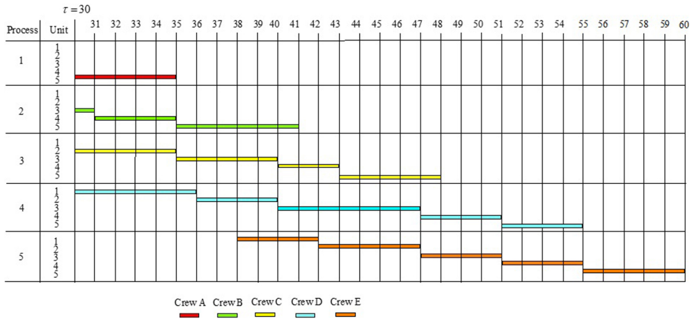
Fig. 1. Project schedule considering the current delay, the production rates of the original resources, and the assumption of resource continuity
