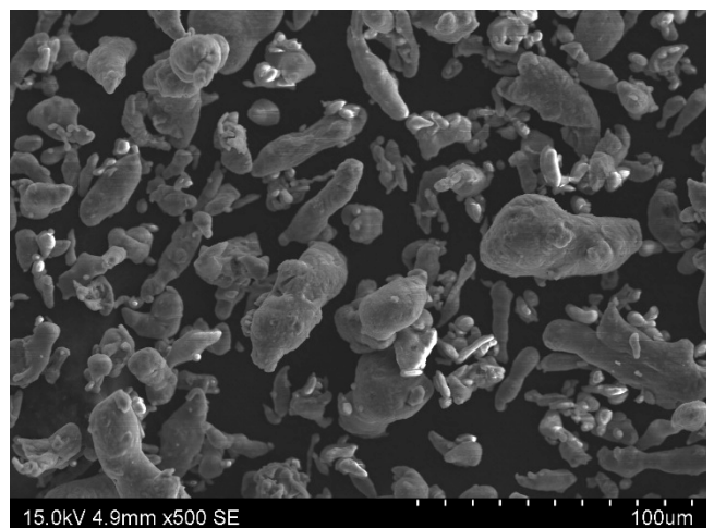
Fig. 1. Morphology of aluminum powder
