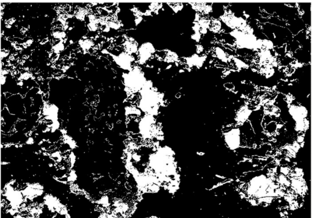
Fig. 6. Representative binary SEM image of composition III (34 at. % Fe), processed using MATLAB for quantitative analysis. Intermetallic regions are shown in white
