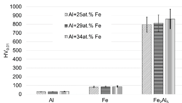
Fig. 9. Vickers microhardness of the sintered samples in different areas: aluminium, iron, and Fe 2 Al 5 intermetallic
