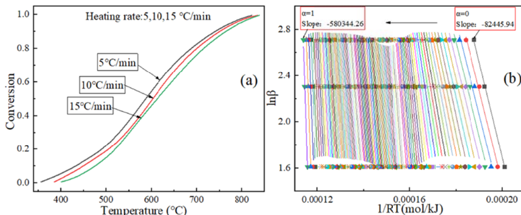
Fig. 5. The growth trend of conversion rate at different heating rates (a). Liner fitting calculation of activation energy at different conversions by FWO model-free method (b)
