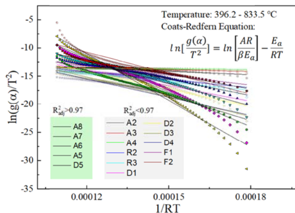
Fig. 7. Model fitting results of heating rates ( 5^\circ\text{C} \cdot \text{min}^{-1} )
