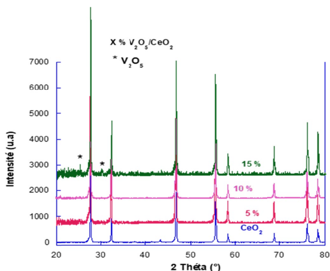
Fig. 2. XRD Diffractograms of CeO 2 and X%V 2 O 5 /CeO 2
