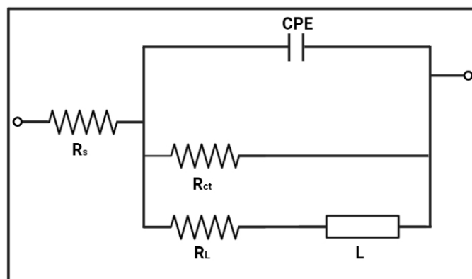
Fig. 5. Impedance spectrum analysis using an electrical equivalent circuit
