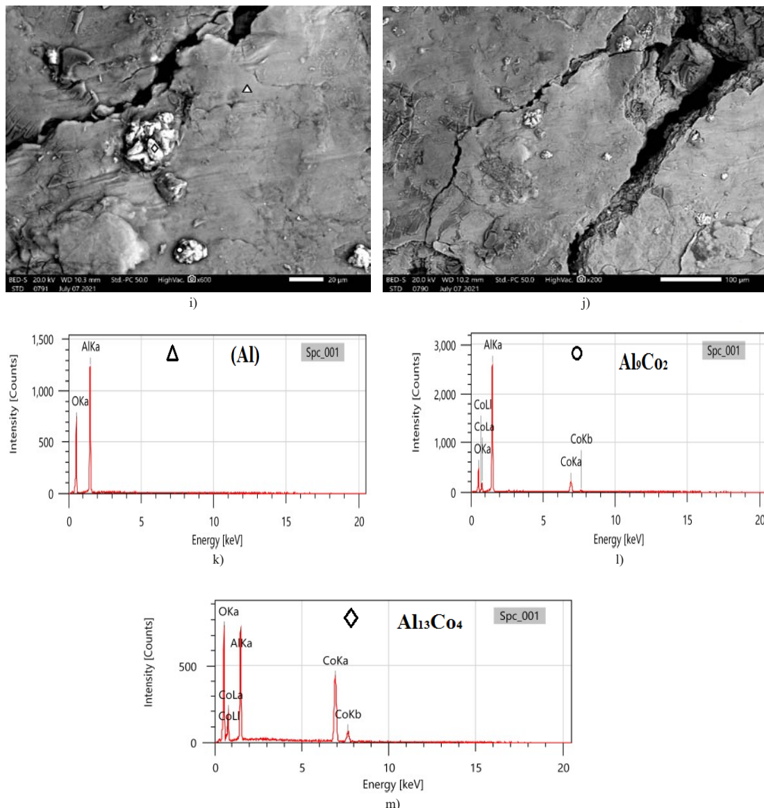
Fig. 9. Microstructure SEM by BSE mode after corrosion testing in HCl medium for the magnifications 20 \mu\text{m} and 100 \mu\text{m} : (a,b) the undoped Al, (c,d,e,f) the ‘SFS-5’ materials sintered at 72 h and 4 h (g,h,i,j) the ‘SFS-0.5’ materials sintered at 72 h and 4 h, (k,l,m) EDS spectra for each phase
