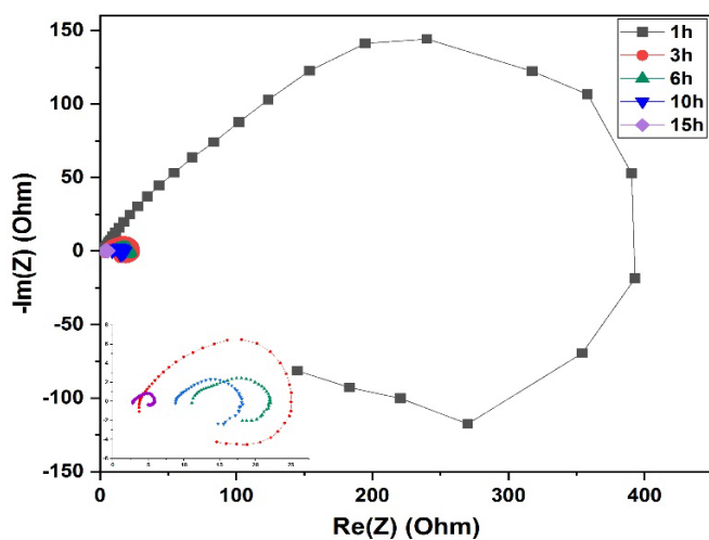
Fig. 7. Nyquist diagram of 'SFS-5'-48 h in 1 M HCl electrolyte at different immersion times
