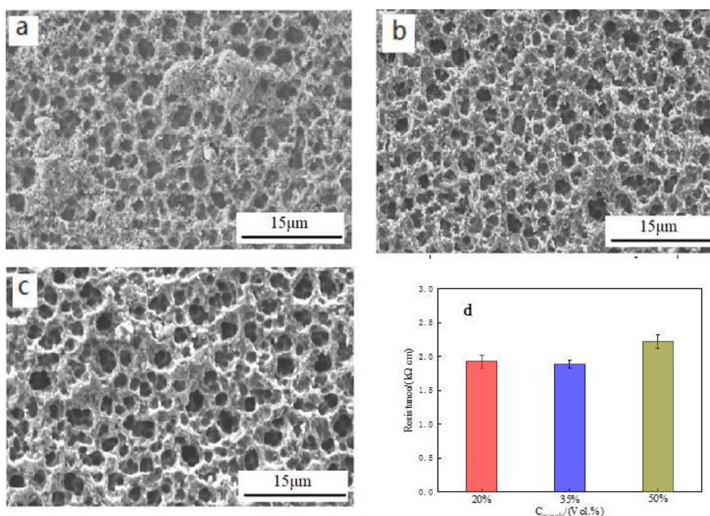
Fig. 3. SEM images of Polypyrrole films obtained in 50 vol% (a), 35 vol% (b) and 20 vol% (c) pyrrole solutions and their specific electrical resistances (d)
