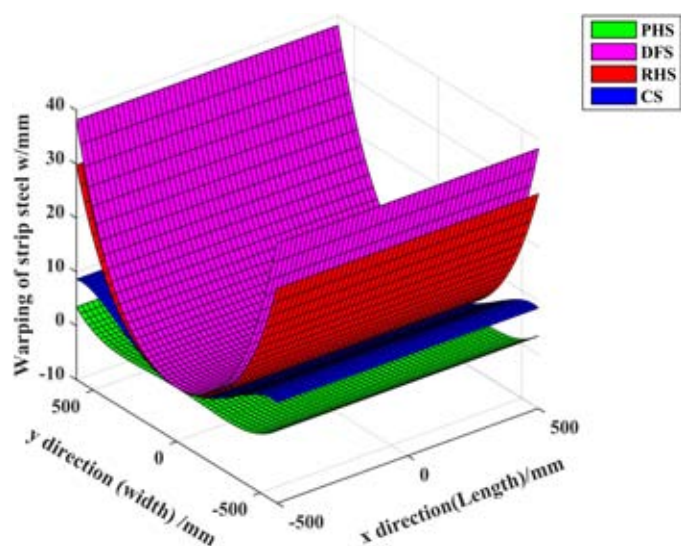
Fig. 15. Strip shape evolving of strip IV
