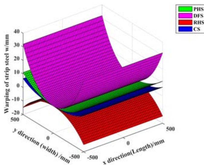
Fig. 16. Strip shape evolving of strip V
