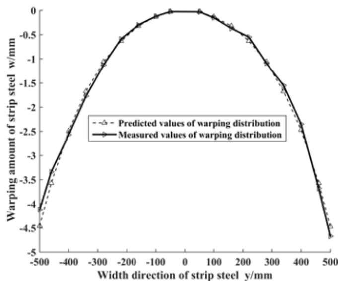
Fig. 9. Strip III warping distribution in unit outlet
