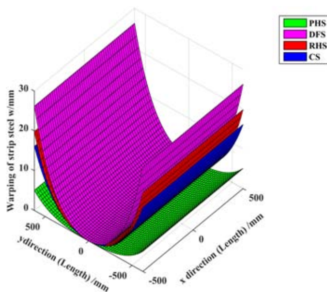
Fig. 12. Strip shape evolving of strip I
