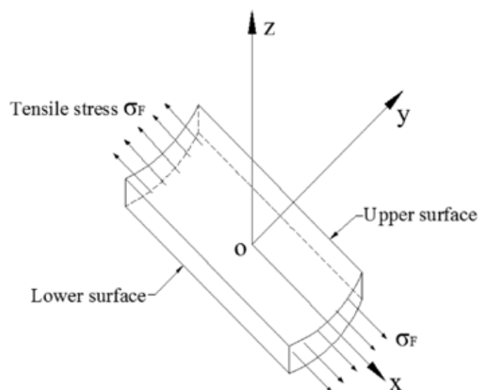
Fig. 4. Force analysis of strip
