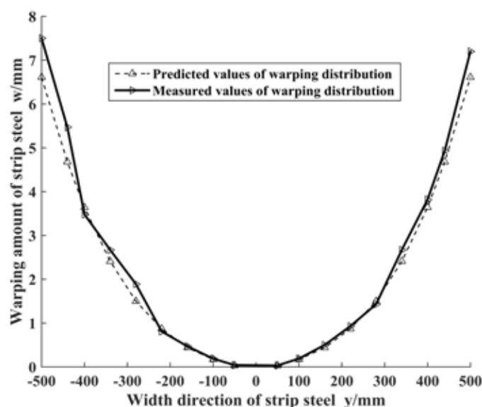
Fig. 11. Strip V warping distribution in unit outlet
