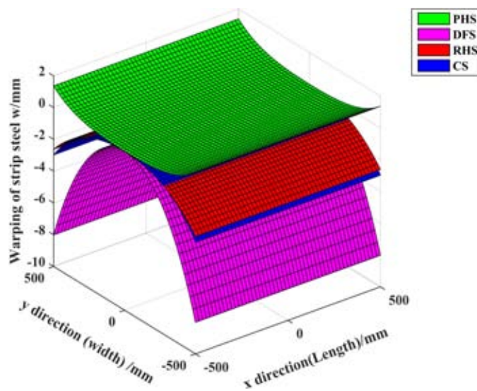
Fig. 14. Strip shape evolving of strip III
