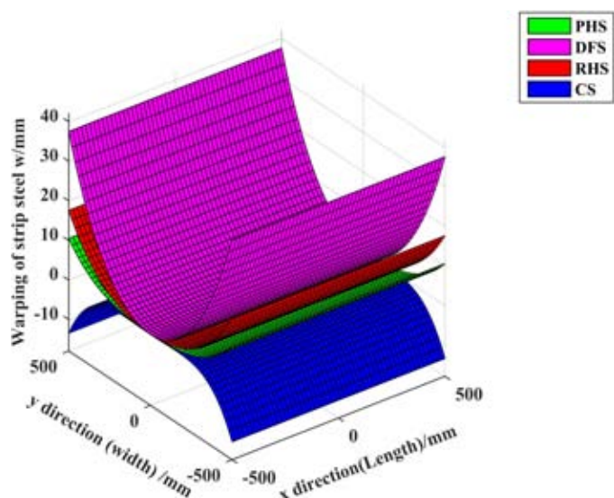
Fig. 13. Strip shape evolving of strip II
