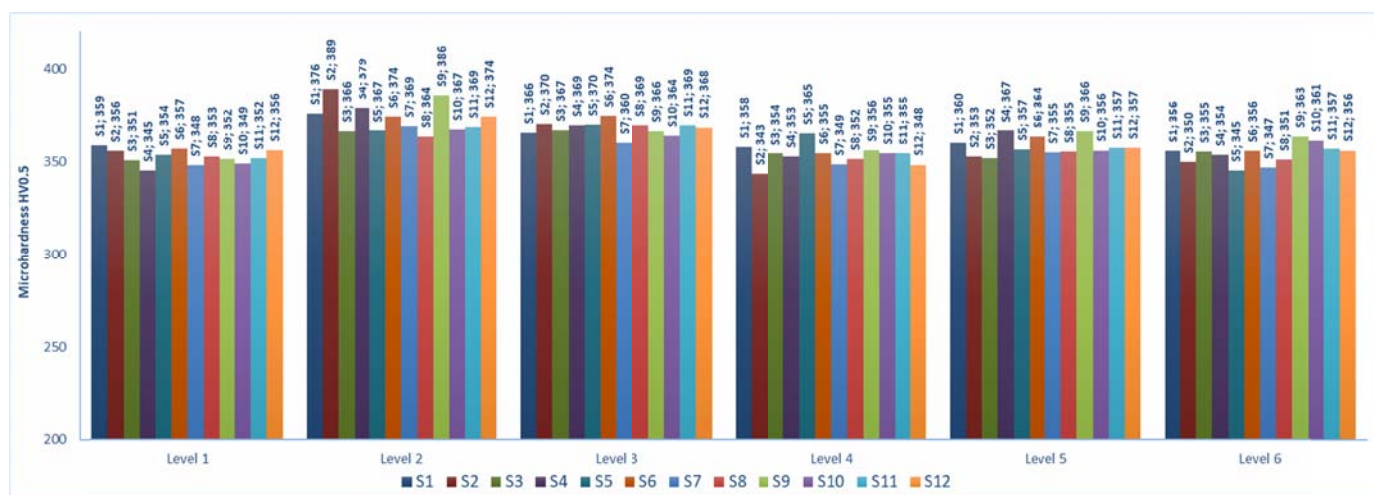
Fig. 15. Average microhardness values of the sample produced with 12 different parameters in 6 layers
