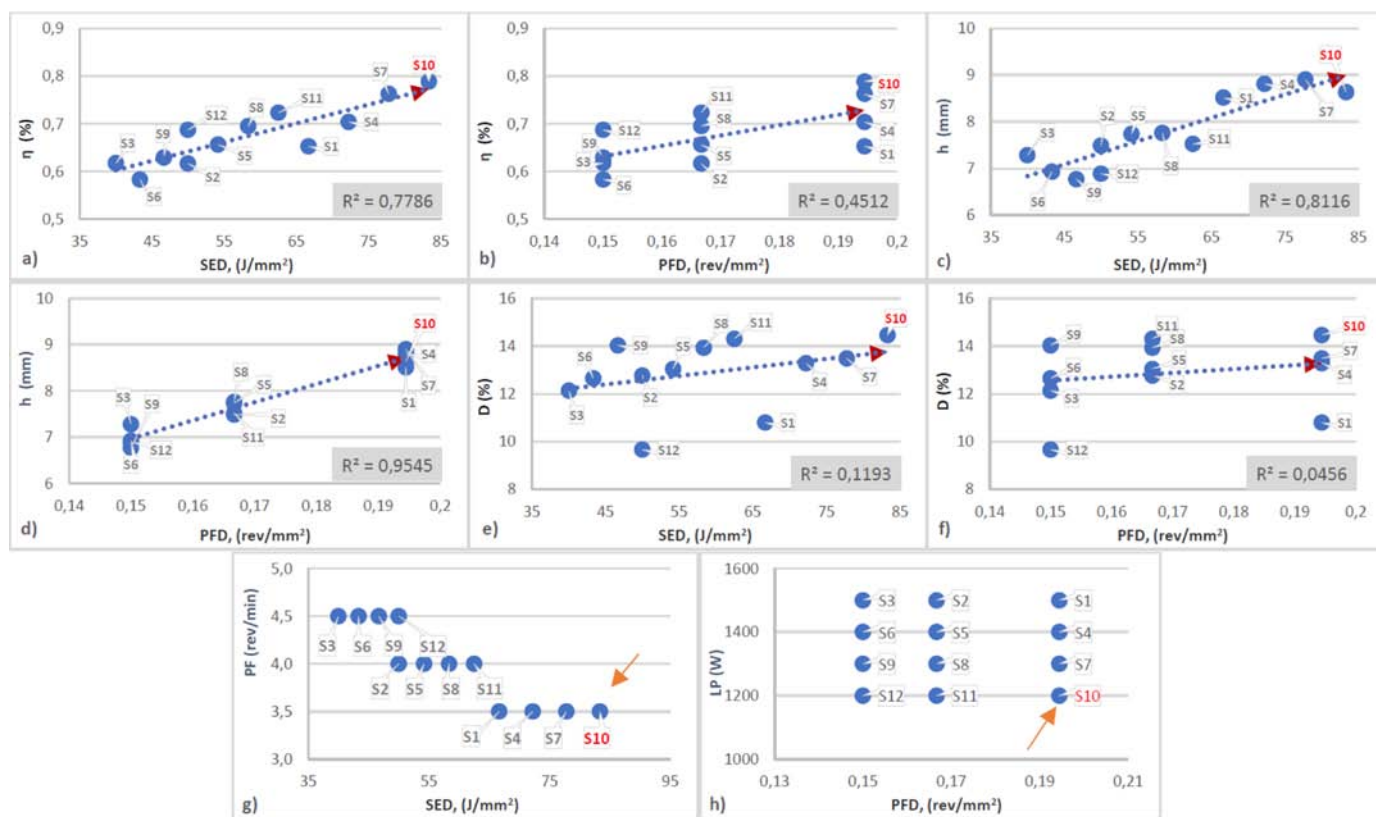
Fig. 6. Effect of SED and PFD on a) and b) \eta , c) and d) h and e) and f) D g) fluctuation of PF with respect to SED h) fluctuation of LP with respect to PFD
