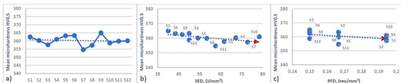
Fig. 16. a) The average hardness distributions of the samples, b) the effects of SED and c) PFD parameters on microhardness
