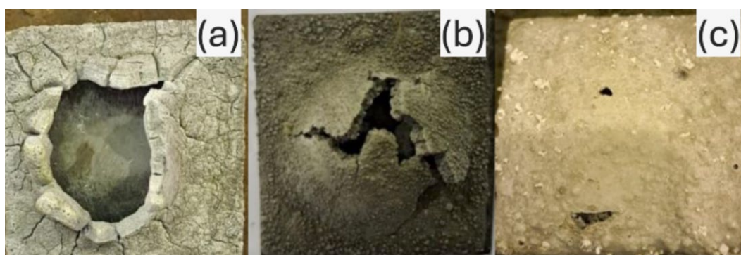
Fig. 6. The coated steel specimens after the fire test: (a) MK-silica fume geopolymer (MS), (b) MK-silica fume-graphite geopolymer (MSG), (c) MK-silica fume-graphite-DSU geopolymer (MSGD) [23]
