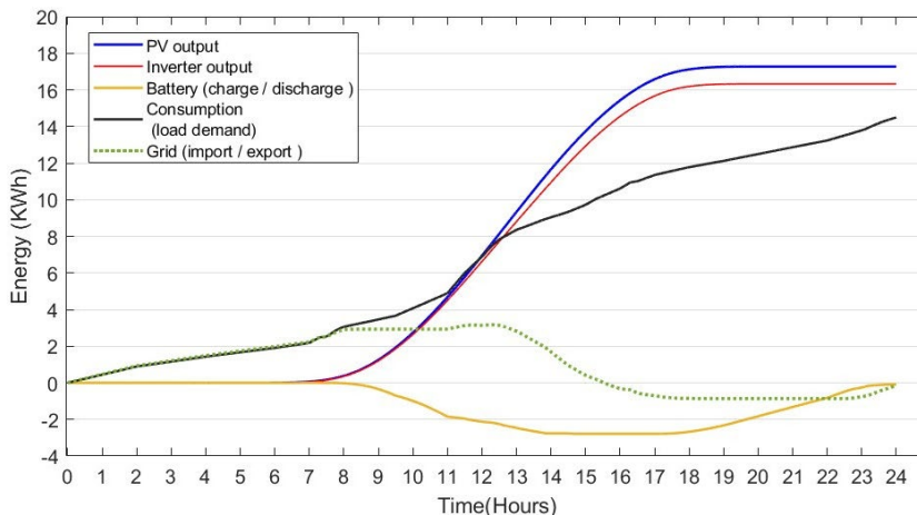
Fig. 9. Daily evolution of the average annual electric energy in different component of the PV system
