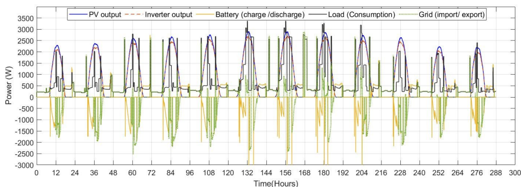
Fig.7. Average monthly power variation over the year for PV generator output, load demand, battery usage, and grid interaction. Positive values for the battery indicate discharging, while negative values indicate charging. For the grid, positive values represent imported power, and negative values represent exported power.
