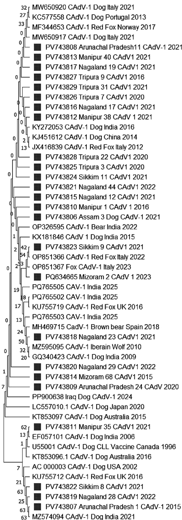
Fig. 3. Phylogenetic analysis of CAHV-1 partial E3 sequences of NEH isolates against reference sequences using the Neighbor-Joining method with 1000 bootstrap replications (MEGA v11.0). The tree is drawn to scale, with branch lengths measured in the number of substitutions per site. Study isolates are marked with blue squares. Bootstrap values \geq 70 indicate strong support. Analysis involved 52 amino acid sequences with 243 positions in the final dataset (pairwise deletion applied).
