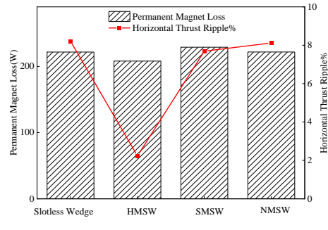
Fig. 9. Permanent magnet loss and horizontal thrust ripple
