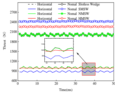
Fig. 8. Electromagnetic thrust
