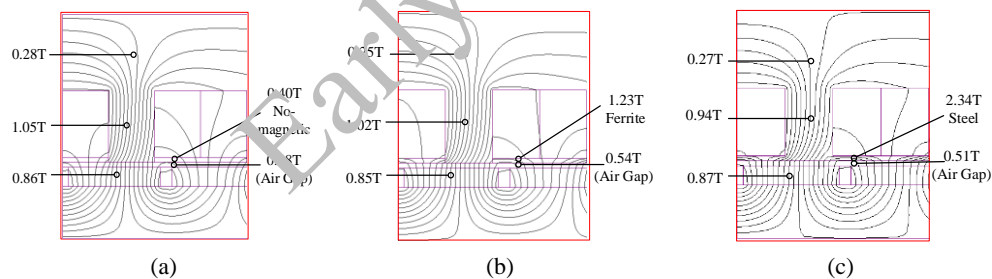
Fig. 4. Distribution of magnetic density: NMSW (a); HMSW (b); SMSW (c)
