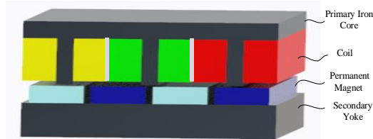
Fig. 2. Topological structure diagram
