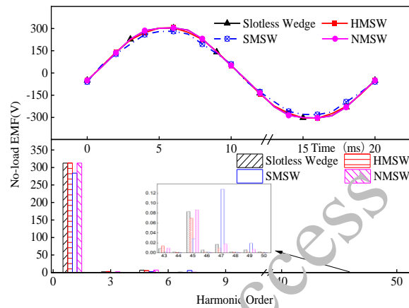
Fig. 6. No-load back EMF and harmonic analysis
