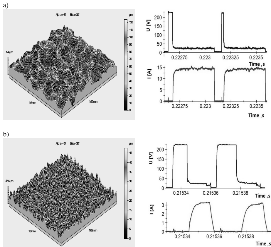
Fig. 4. Stereometric image of the surface with recorded wave forms current voltage characteristics after EDM: a) U_c = 25 \text{ V} , I_c = 14,3 \text{ A} , t_{\text{on}} = 80 \text{ } \mu\text{s} , t_{\text{off}} = 18 \text{ } \mu\text{s} , b) U_c = 25 \text{ V} , I_c = 3,2 \text{ A} , t_{\text{on}} = 11 \text{ } \mu\text{s} , t_{\text{off}} = 150 \text{ } \mu\text{s}
