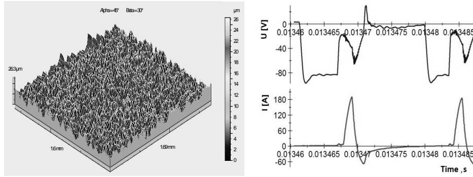
Fig. 5. Stereometric image of the surface with recorded waveforms current voltage characteristics after WEDM: U_c = 25 V, I_c = 185 A, I_w = 6 A, t_{on} = 1 µs, t_{off} = 12 µs
