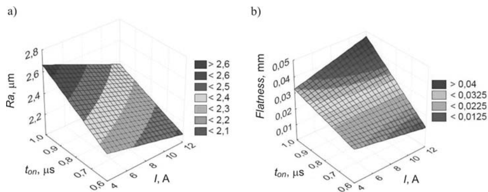
Rys. 7. The dependence of surface texture parameters after WEDM from pulse time t_{on} and the current I_w
