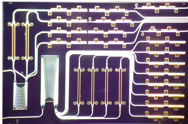
Fig. 7. FTTH transmitters after Ref. 13. The 8-channel circuit comprises an array of eight DBR lasers (right side of the chip). Four channels are digitally modulated by Mach-Zehnder modulators (downstream), four channels provide CW power for the upstream signals
