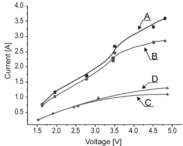
Fig. 6. Measured current-voltage characteristics for: laser diode driven with different current pulses (A: t_i = 20 ns and B: t_i = 2 \mu s) and two QC laser models with resistance of 3.3 \Omega and 1 \Omega (C,D)
