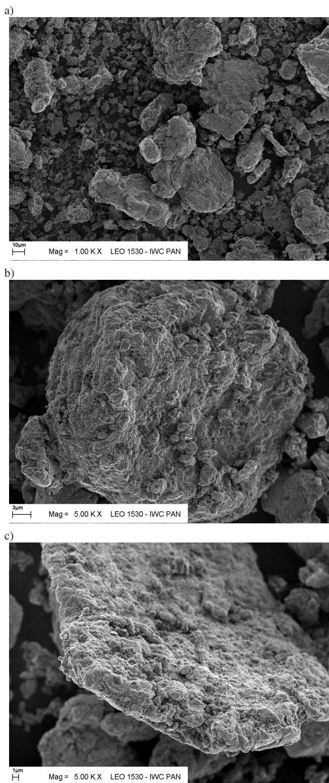
Fig. 2. SEM images of 80Cu-20AlN powder mixtures
