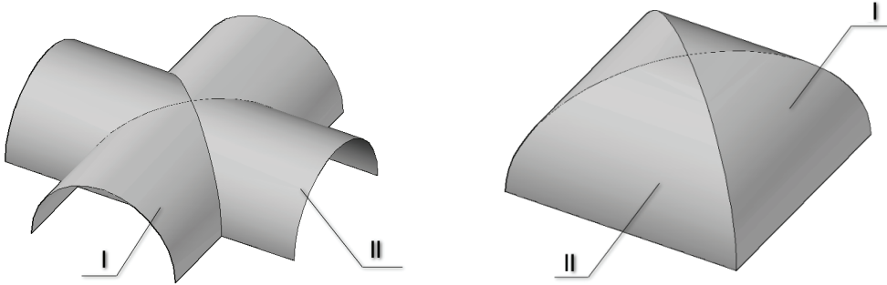
Fig. 2. Cylindrical shells I-II in the form of perpendicular intersection of the four-wall dome over the Gdynia Seaport Building
