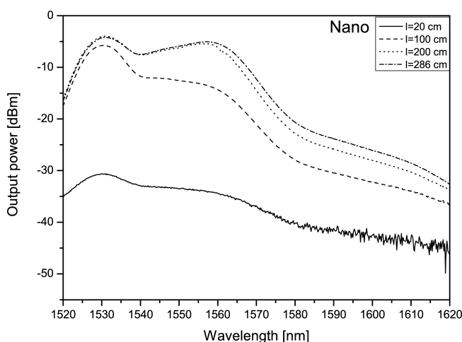
Fig. 14. Backward ASE of the NANO fiber
