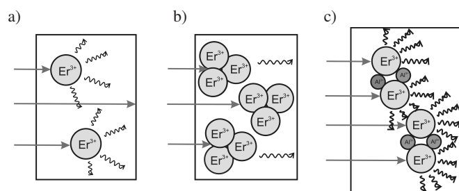
Fig. 2. A schematic image of the influence of Er clusters and nanocrystals in a disordered glass matrix on luminescence intensity: a) RE ions in low concentration distributed in a silica glass matrix produce weak luminescence, b) increased concentration of RE ions results in the formation of clusters decreasing the luminescence, c) the effect of nanoparticles results in higher concentration of RE ions well distributed in the glass matrix and improving the luminescence properties of the material
