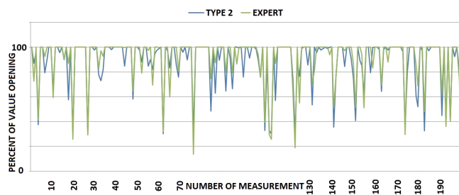
Fig. 13. Angles of the ammonia valve opening evaluated the type-2 FLS (blue) and proposed by a human expert (green). Type-2 inference: the min implication. Compare Table 4, row 2
