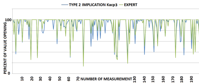
Fig. 15. Angles of the ammonia valve opening evaluated the type-2 FLS (blue) and proposed by a human expert (green). Type-2 inference: implication I_{K_3} . Compare Table 4, row 7
