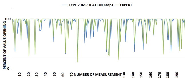
Fig. 14. Angles of the ammonia valve opening evaluated the type-2 FLS (blue) and proposed by a human expert (green). Type-2 inference: implication I_{K_1} . Compare Table 4, row 5
