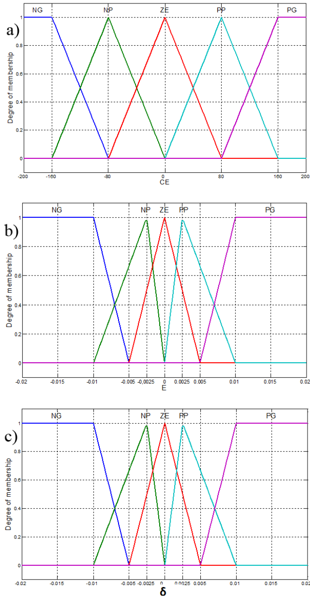
Figure 10. Membership function.
